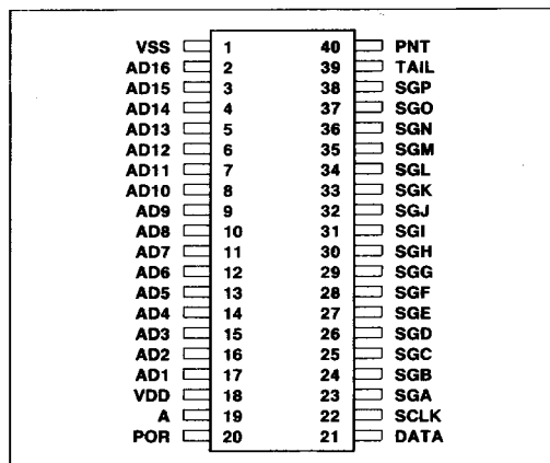
10951 Pin Configuration
