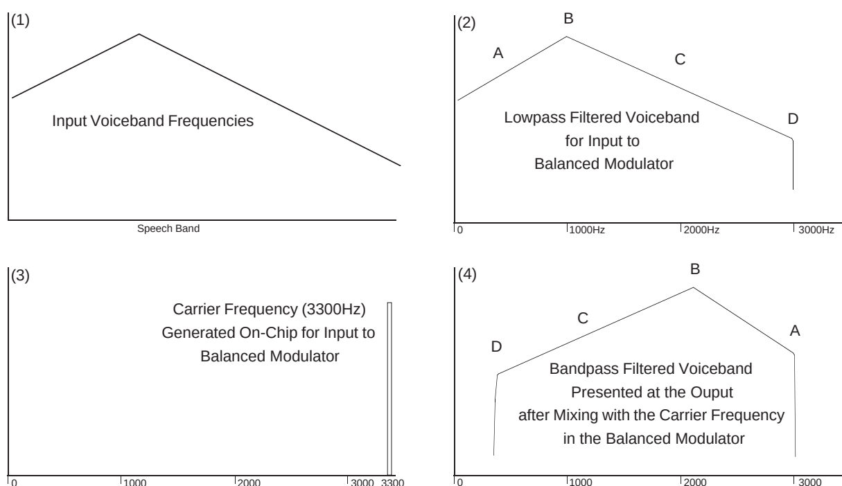
Fig.5 A Pictorial Explanation of the FX118 "Scramble Operation"
