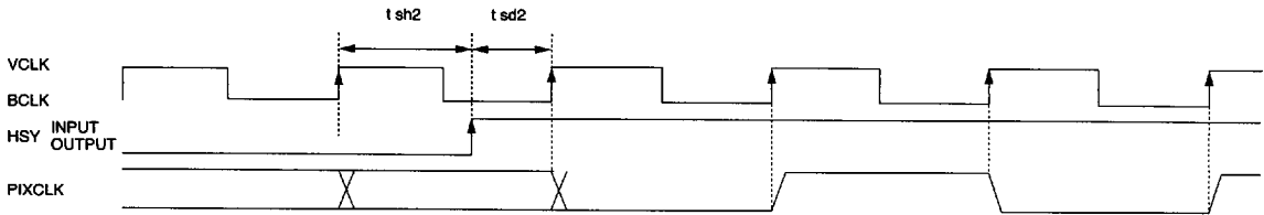
Fig. 8 PIXCLK output timing (when CLKSW = high)
