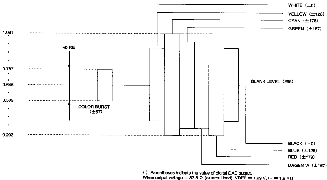
Fig. 2 NTSC C (chroma) signal output level
