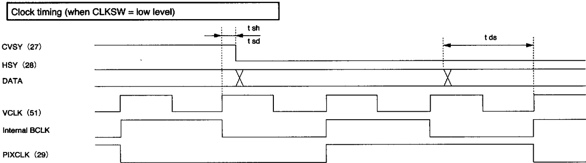
Fig. 5 Clock timing and data input timing
