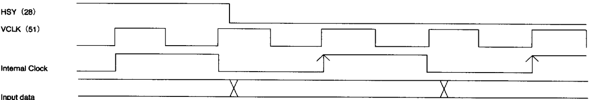
Fig. 2-3-1 Clock timing (CLKSW is at the low level)
