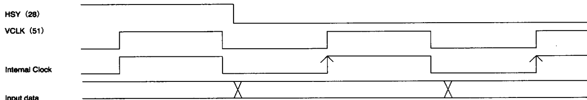
Fig. 2-3-2 Clock timing (CLKSW is at the high level)
