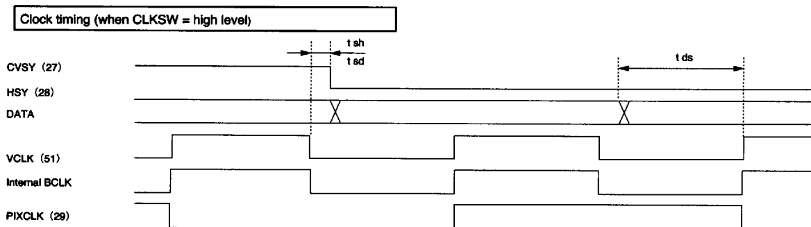
Fig. 6 Clock timing and data input timing
