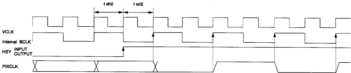
Fig. 9 PIXCLK output timing (when CLKSW = low)
