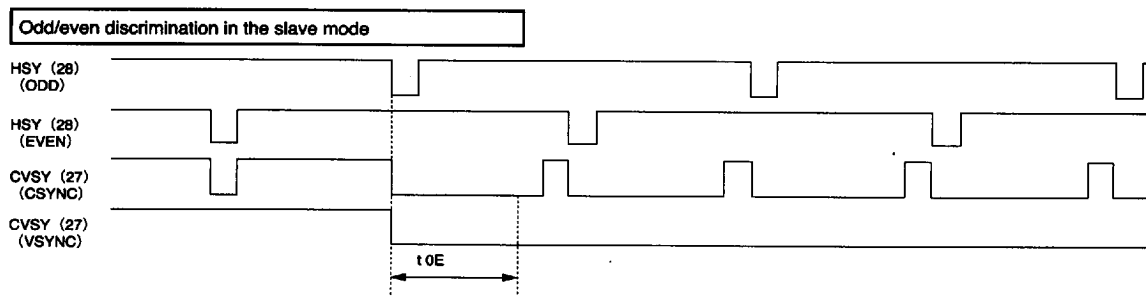
Fig. 7 Odd/even discrimination timing in the slave mode
