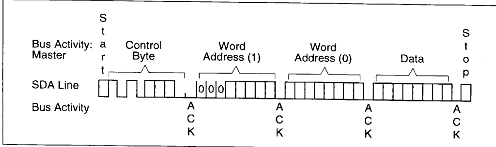
FIGURE 4-1: BYTE WRITE
