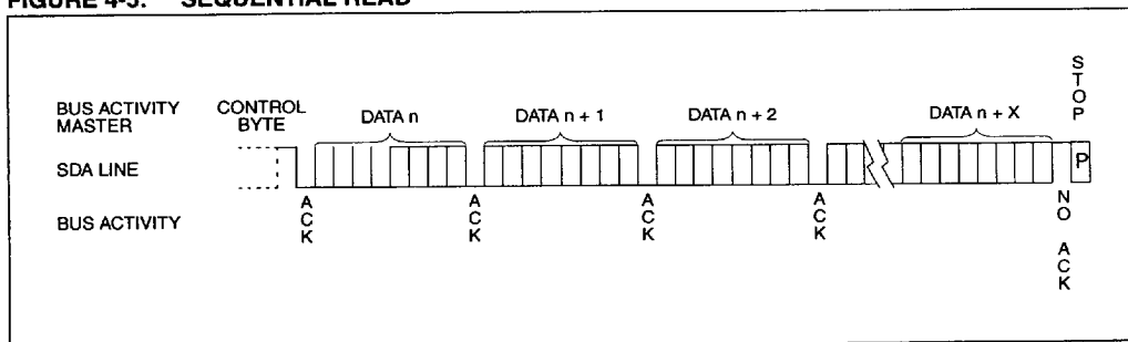
FIGURE 4-5: SEQUENTIAL READ
