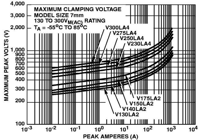
FIGURE 4. CLAMPING VOLTAGE FOR V130LA2 - V300LA4
