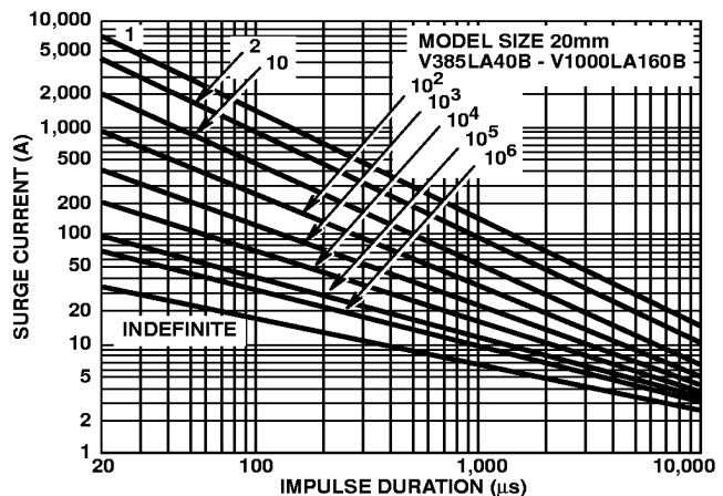
FIGURE 19. SURGE CURRENT RATING CURVES FOR V385LA40B - V1000LA160B
