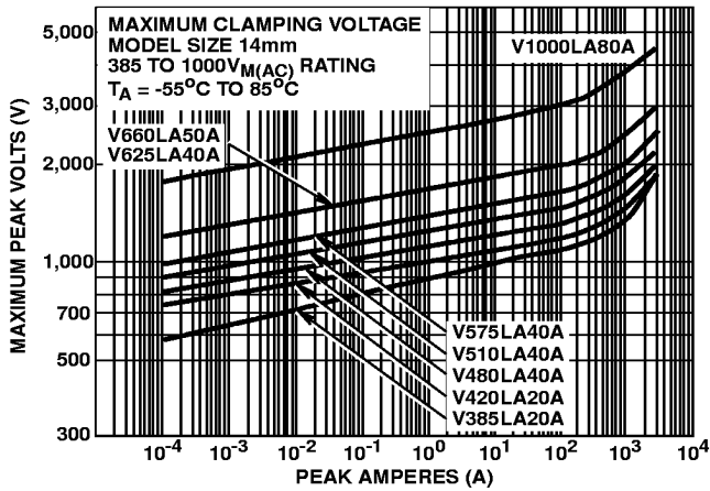
FIGURE 9. CLAMPING VOLTAGE FOR V385LA20A - V1000LA80A
