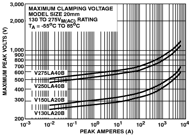
FIGURE 11. CLAMPING VOLTAGE FOR V130LA20B - V275LA40B
