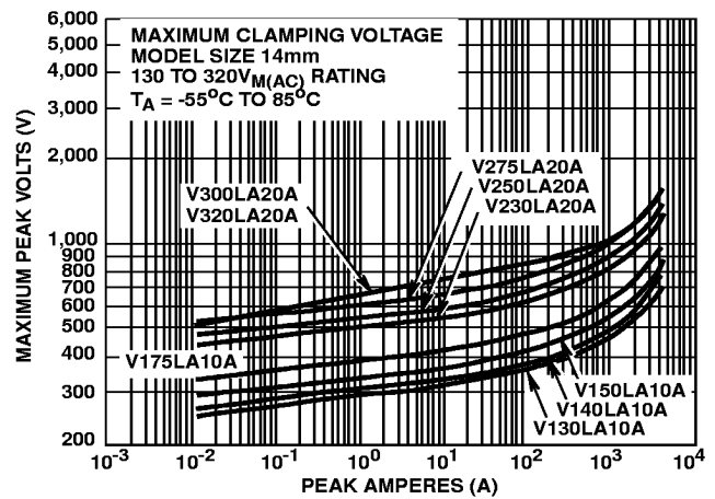
FIGURE 8. CLAMPING VOLTAGE FOR V130LA10A - V320LA20A
