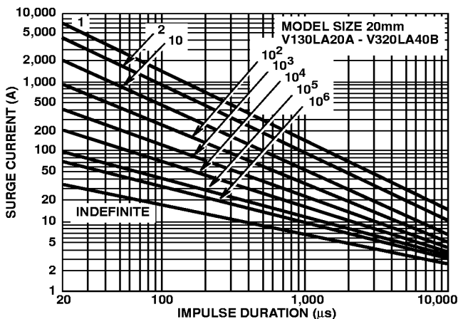
FIGURE 18. SURGE CURRENT RATING CURVES FOR V130LA20A - V320LA40B
