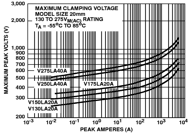
FIGURE 10. CLAMPING VOLTAGE FOR V130LA20A - V275LA40A
