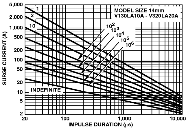
FIGURE 16. SURGE CURRENT RATING CURVES FOR V130LA10A - V320LA20A
