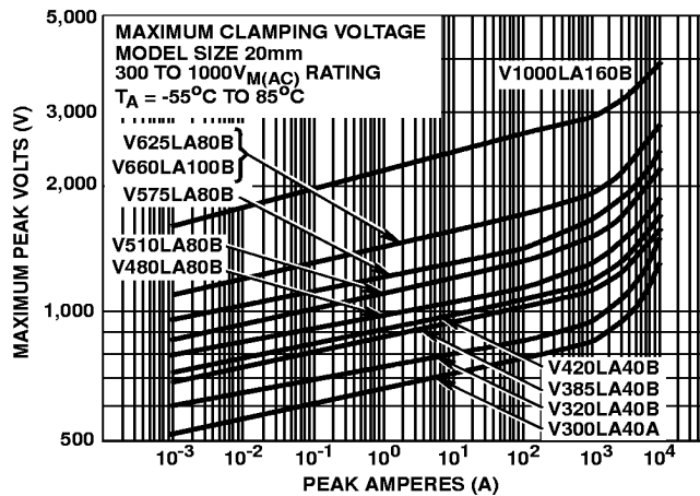
FIGURE 13. CLAMPING VOLTAGE FOR V300LA40A - V1000LA160B
