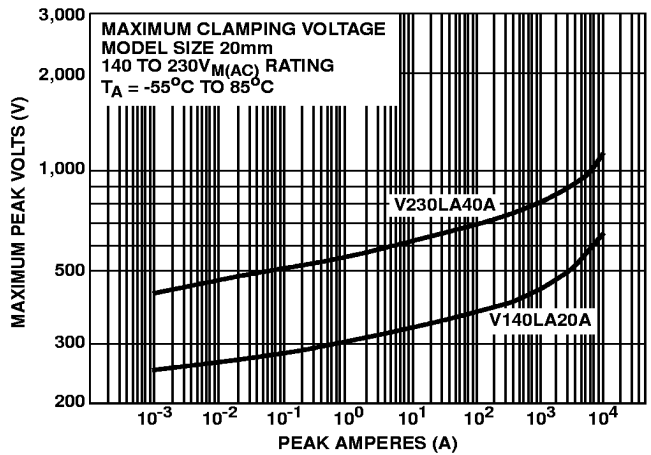
FIGURE 12. CLAMPING VOLTAGE FOR V140LA20A - V230LA40A
