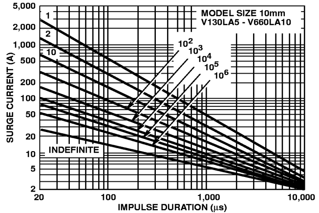
FIGURE 15. SURGE CURRENT RATING CURVES FOR V130LA5 - V660LA10
