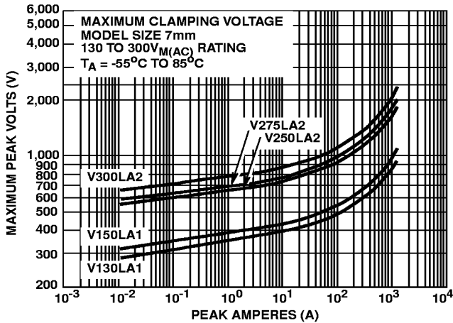
FIGURE 3. CLAMPING VOLTAGE FOR V130LA1 - V300LA2
