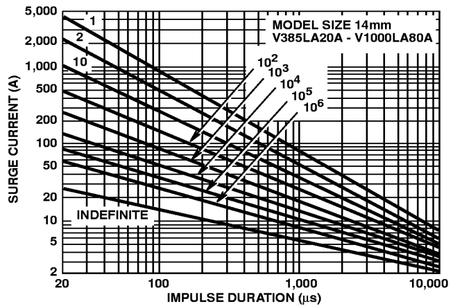
FIGURE 17. SURGE CURRENT RATING CURVES FOR V385LA20A - V1000LA80A
