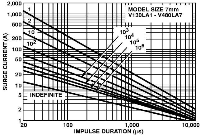
FIGURE 14. SURGE CURRENT RATING CURVES FOR V130LA1 - V480LA7
