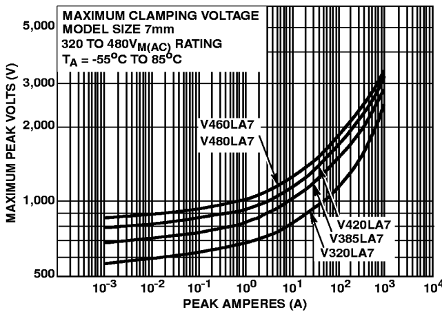
FIGURE 5. CLAMPING VOLTAGE FOR V320LA7 - V480LA7
