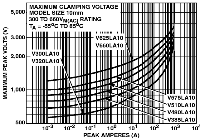
FIGURE 7. CLAMPING VOLTAGE FOR V300LA10 - V660LA10
