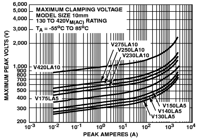
FIGURE 6. CLAMPING VOLTAGE FOR V130LA5 - V420LA10
