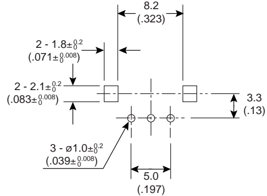
P.C.B. Mounting Hole Detail
