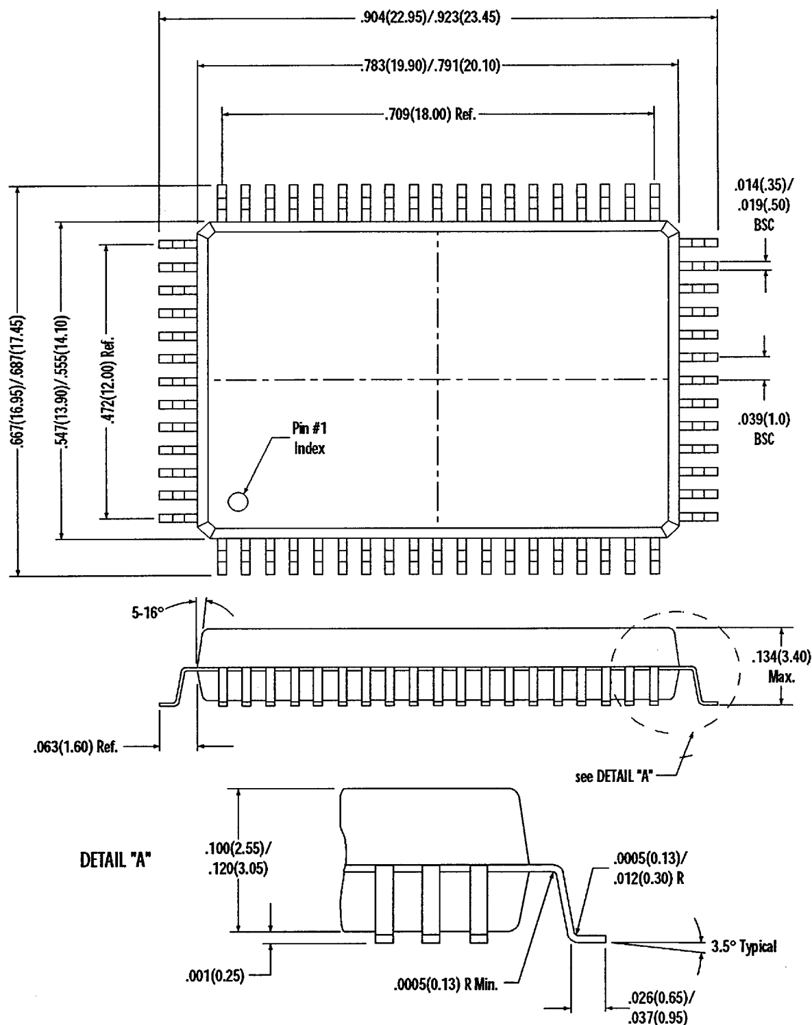
Figure 16. Q2240I-2S1 and Q2240I-3S1 64-pin PQFP Package Outline
