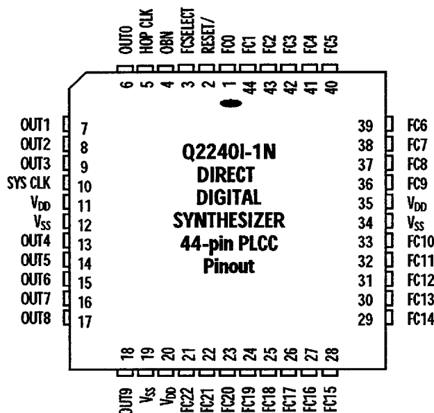
Figure 6. Q2240I-1N (24-bit Parallel Interface) Pinout Diagram
