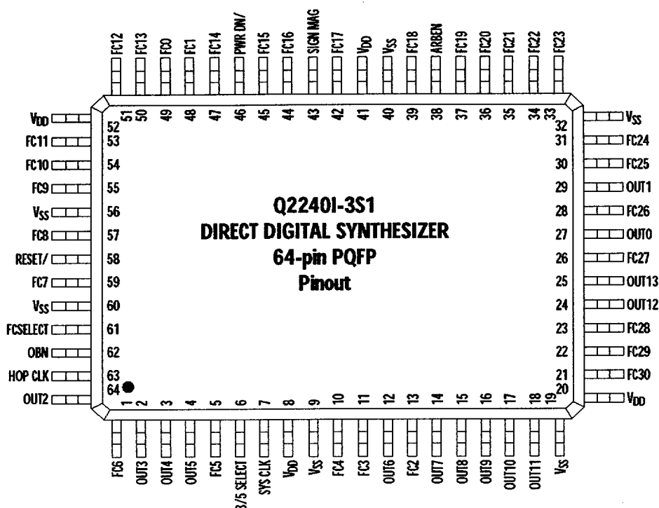
Figure 8. Q2240I-3S1 (32-bit Parallel Interface) Pinout Diagram
