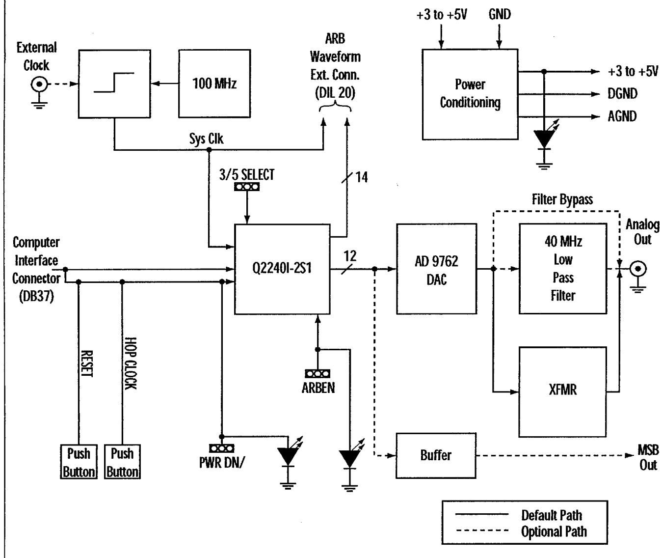
Figure 17. Q0340-2 Functional Block Diagram
