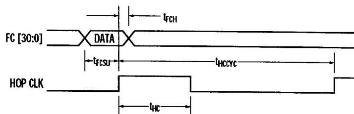
Figure 11. Q2240I-1N and Q2240I-3S1 Asynchronous Parallel Interface (FCSELECT = "1") Timing Diagram
