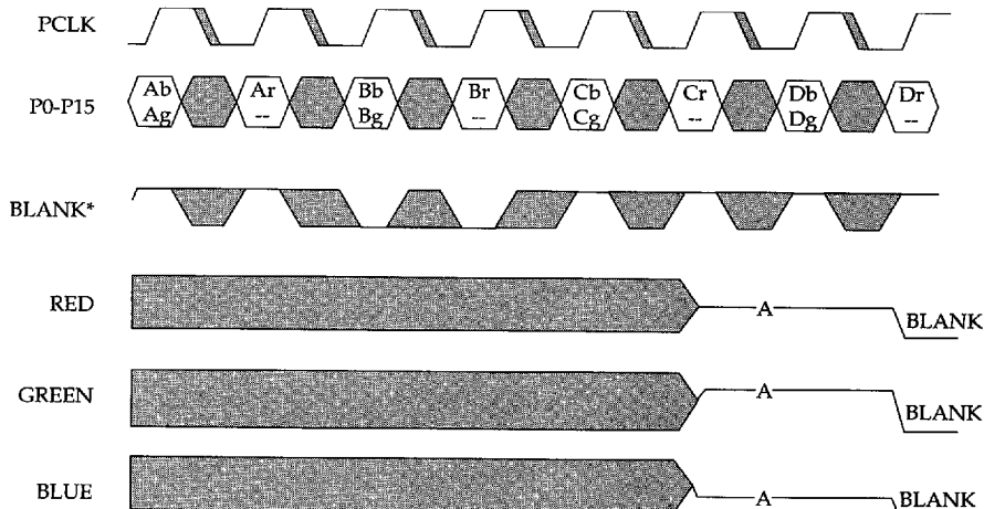
System Timing - 16-bit Direct True Color, Mode 7
