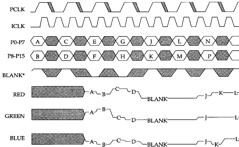
System Timing - Multiplexed 8-bit Pseudo Color, Mode 4
