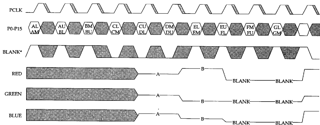
System Timing - 24-bit Packed Color, Mode 8
