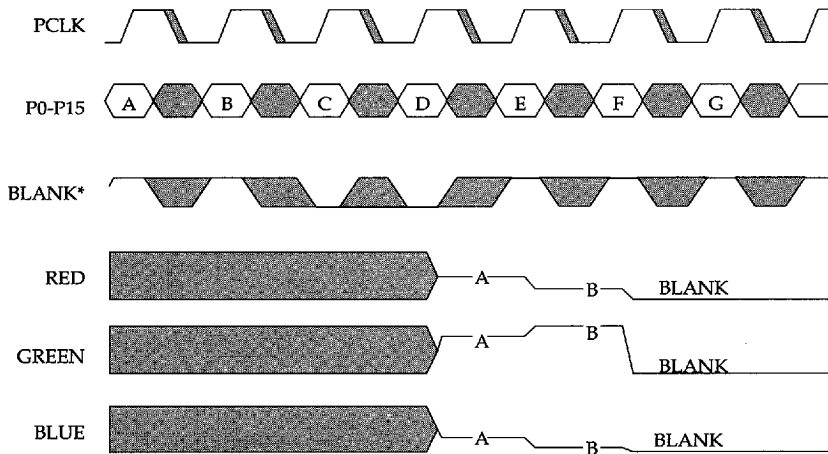
System Timing - 16-bit Color, Mode 5 (5,5,5) and 6 (5,6,5)
