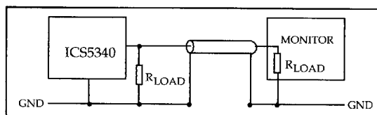
Figure 1 - Double Termination
