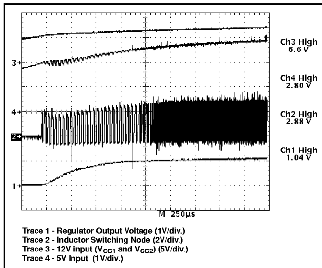
Figure 2: CS-5157H demonstration board startup in response to increasing 12V and 5V input voltages. Extended off time is followed by normal off time operation when output voltage achieves regulation to the error amplifier output.
