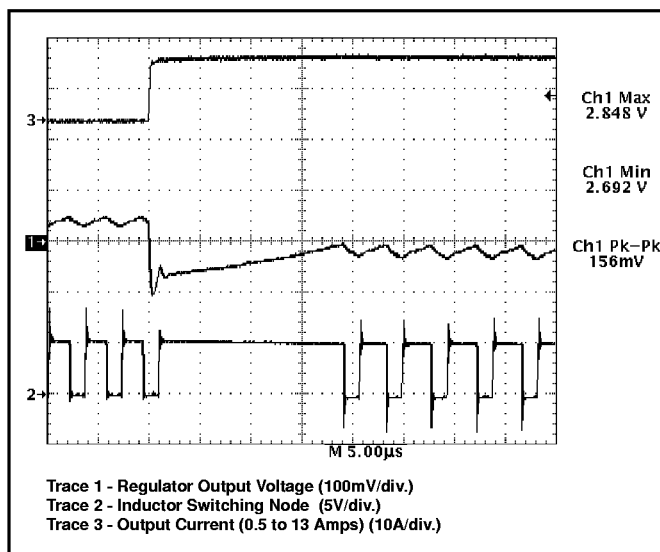
Figure 8: CS-5157H demonstration board response to 13A load turn on (output set for 2.8V). Upon completing a normal off time, the V^2 ™ control loop immediately connects the inductor to the input voltage, providing 100% duty cycle. Regulation is achieved in less than 20μs.
