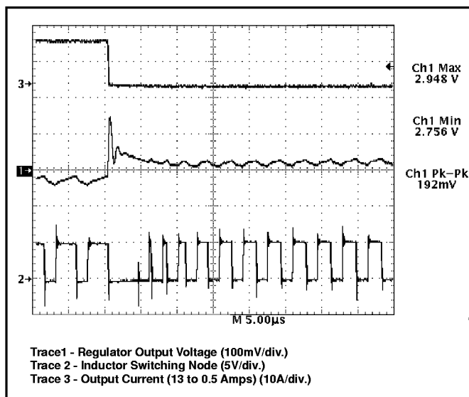
Figure 9: CS-5157H demonstration board response to 13A load turn off (output set for 2.8V). V^2 ™ control topology immediately connects inductor to ground, providing 0% duty cycle. Regulation is achieved in less than 10μs.
