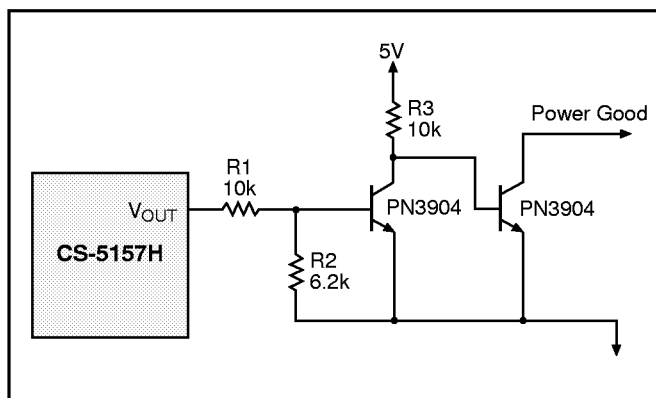
Figure 15: Implementing Power Good with the CS-5157H.
