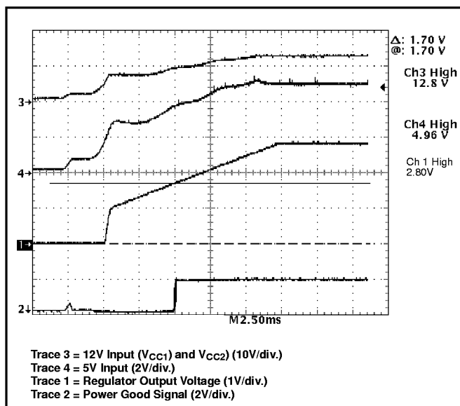
Figure 16: CS-5157H demonstration board during power up. Power Good signal is activated when output voltage reaches 1.70V.
