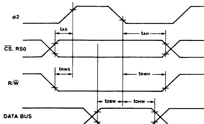
Microprocessor Write Cycle
