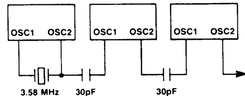
Figure 8. Common Crystal Connection
