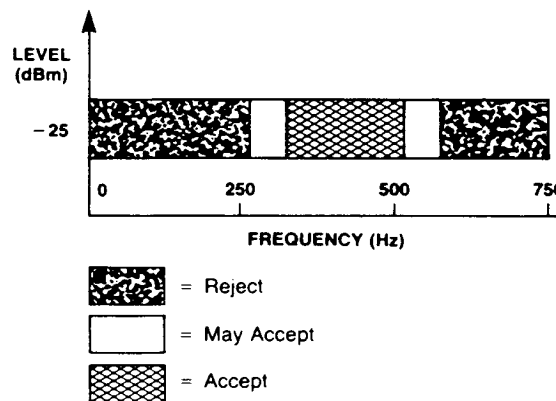
Figure 6. Call Progress Response
