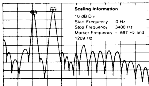
Figure 7. Spectrum Plot
