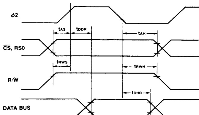
Microprocessor Read Cycle
