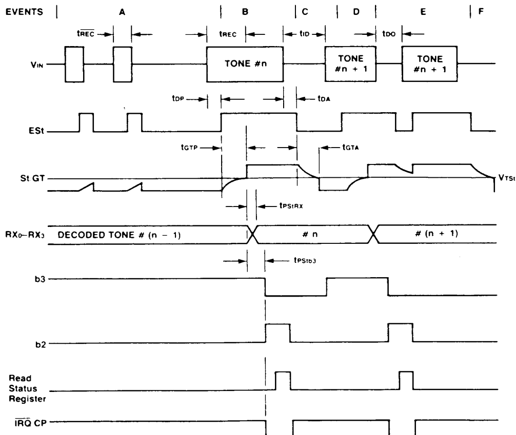
General Transceiver Timing
