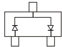
BAV199T Marking: 52
