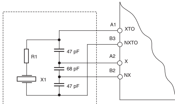
Figure 5-2. Application Example Using a GPS Crystal With ESR Typically ≠ 12Ω (See Table 5-2 on page 27 )
