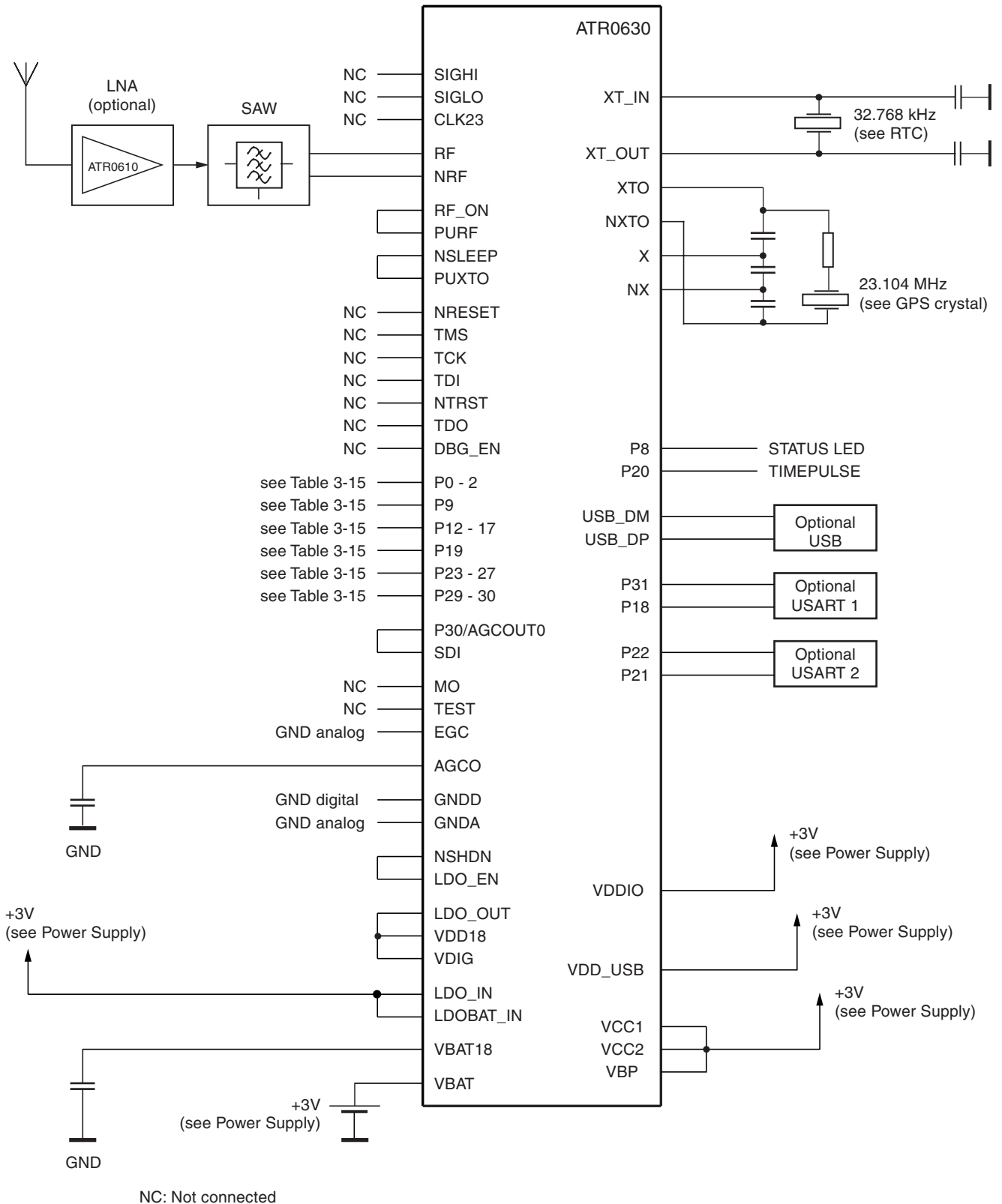
Figure 3-2. Example of an External Connection (ATR0630)
