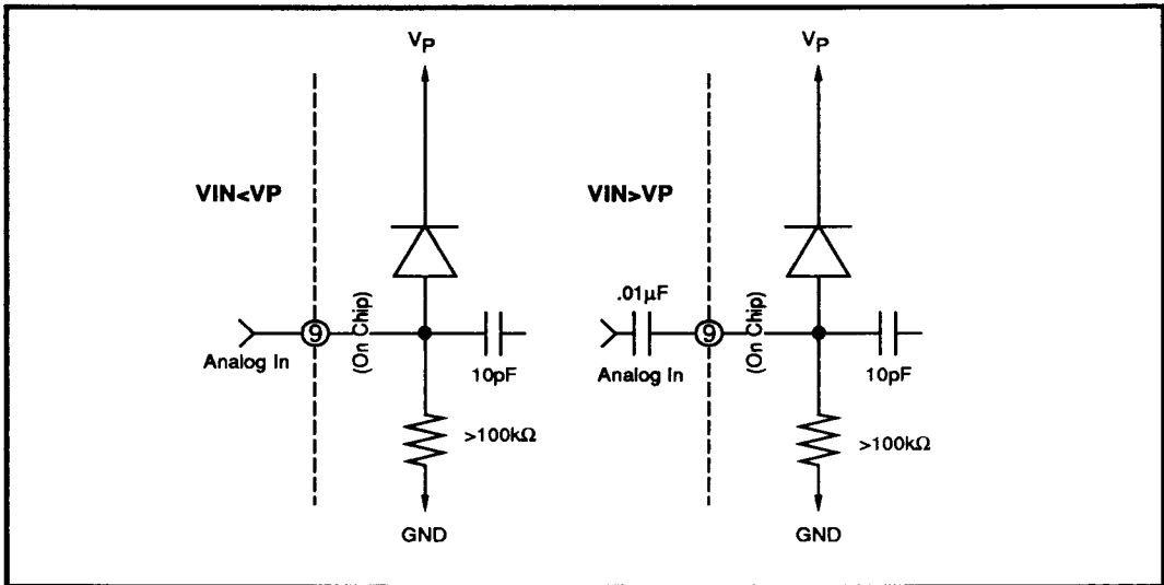
FIGURE 1: Input Coupling
