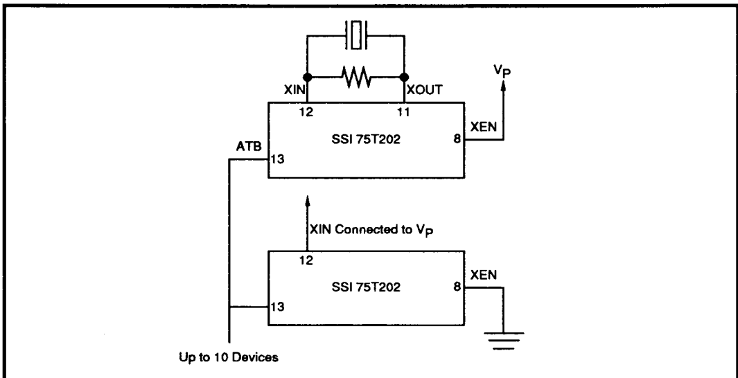
FIGURE 2: Crystal Connections
