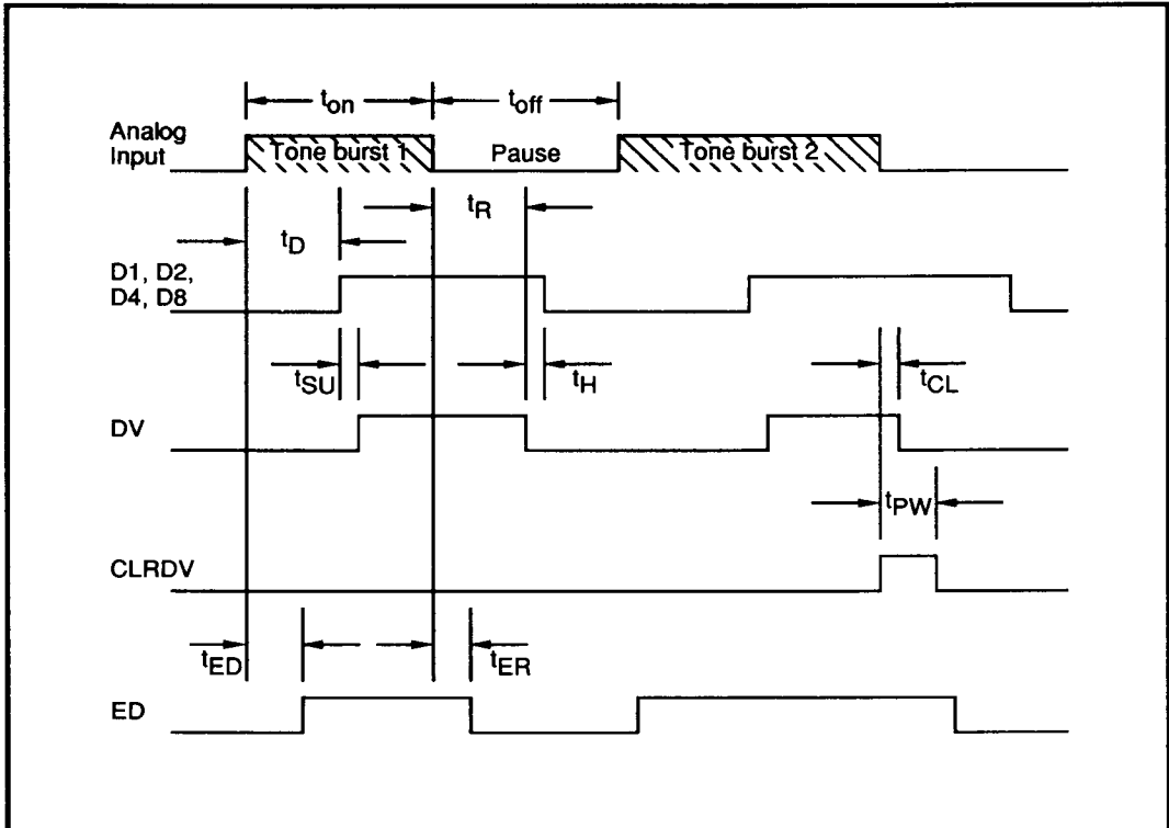
FIGURE 4: Timing Diagram
