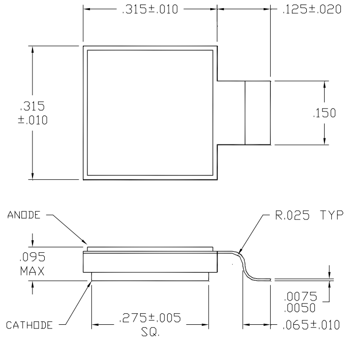
CASE OUTLINE: SED75KE30
