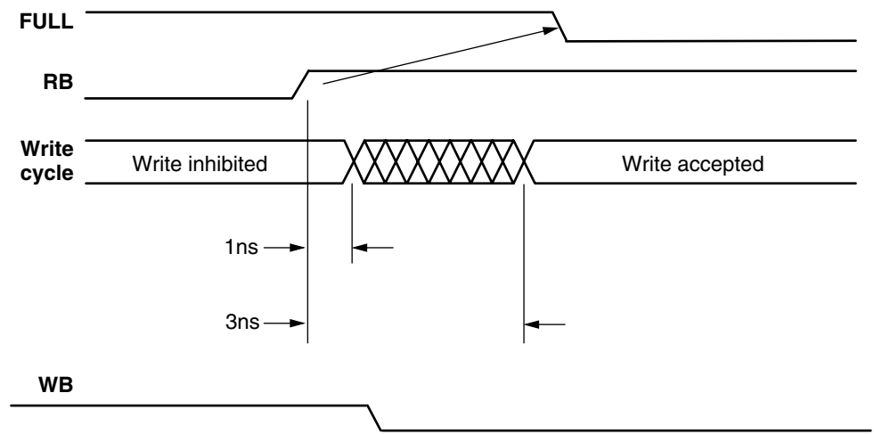
Figure 19 • Write Timing Diagram
