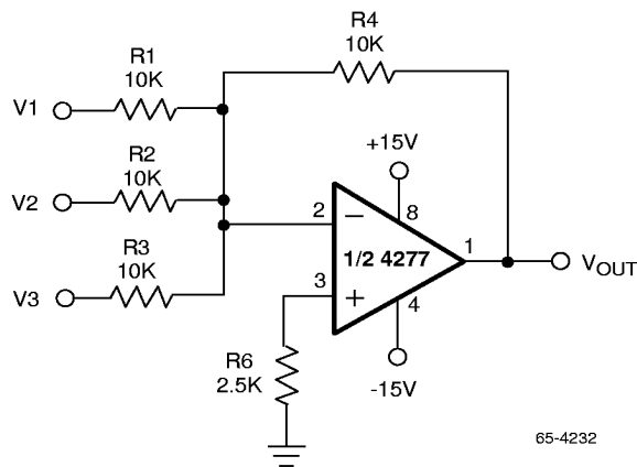
Figure 1. Adjustment-Free Precision Summing Amplifier
