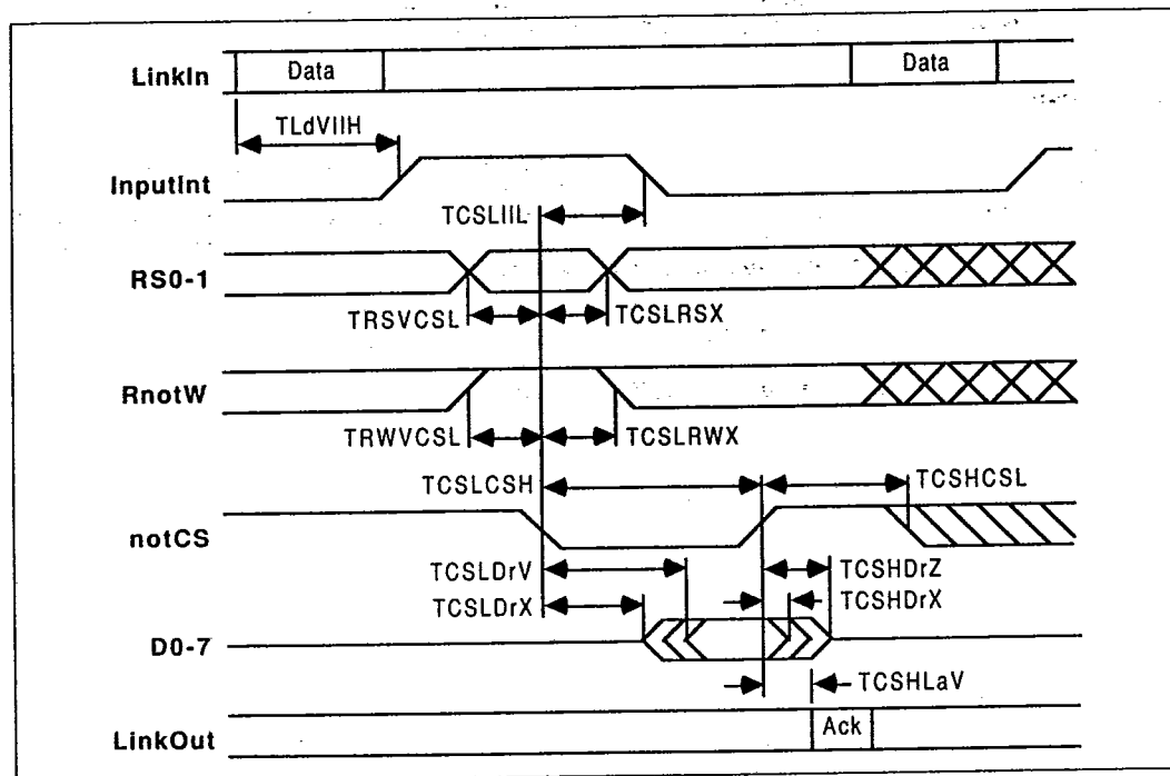
Figure 6.1: IMS C011 Mode 2 read parallel data from link adaptor
