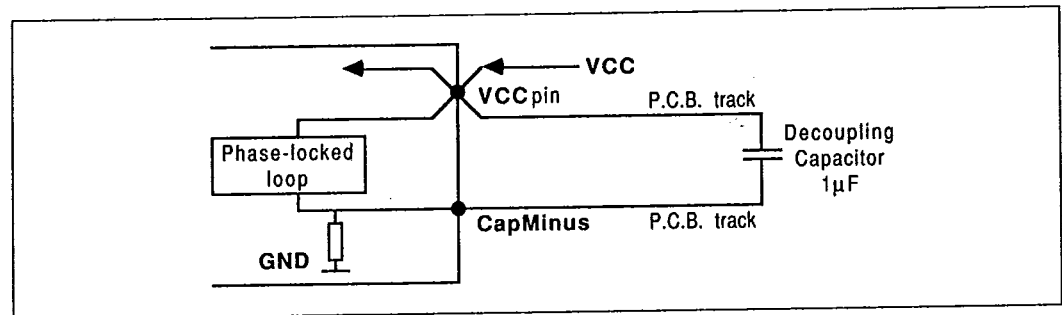
Figure 3.1: Recommended PLL decoupling
