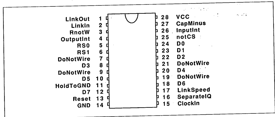
Figure 8.4: IMS C011 Mode 2 pinout
