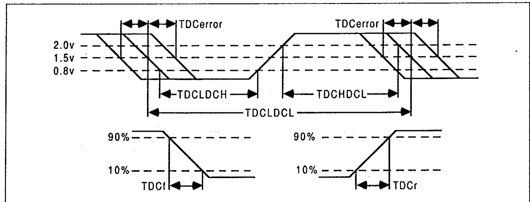
Figure 3.2: ClockIn timing
