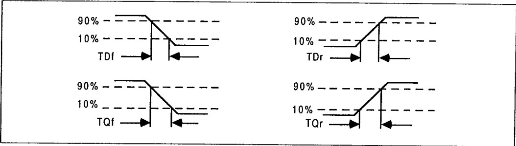
Figure 7.3: IMS C011 input and output edge timing
