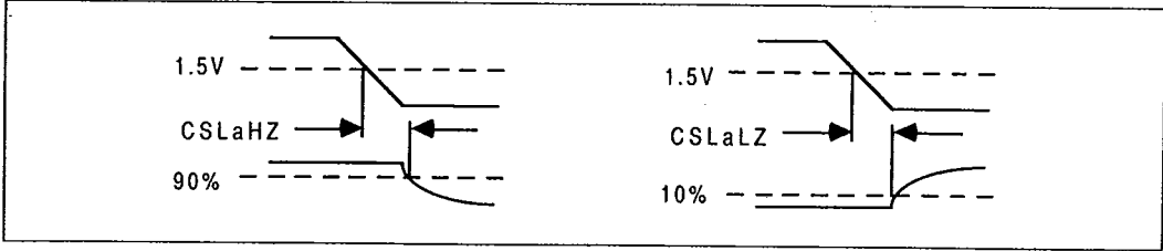
Figure 7.4: IMS C011 tristate timing relative to notCS
