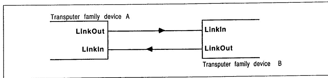
Figure 4.4: Links directly connected
