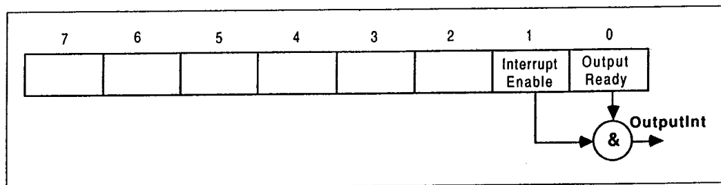
Figure 6.4: IMS C011 Mode 2 output status register
