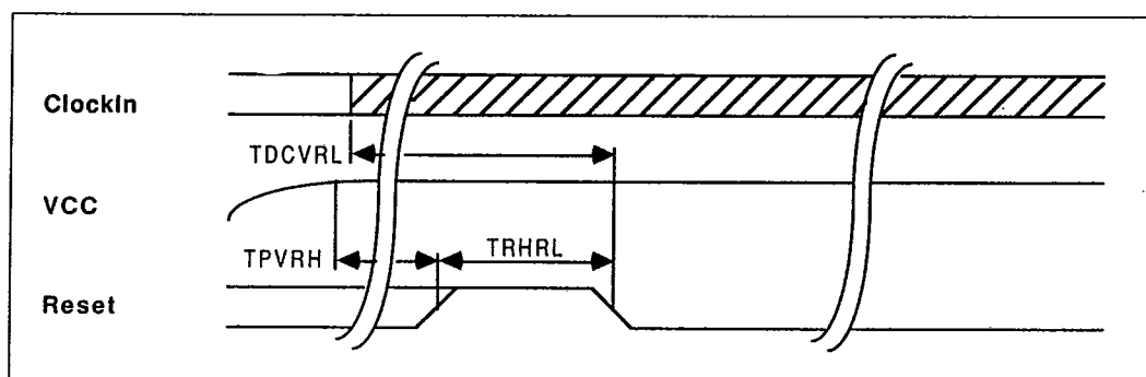
Figure 3.3: Reset timing
