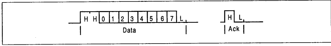
Figure 4.1: IMS C011 link data and acknowledge packets
