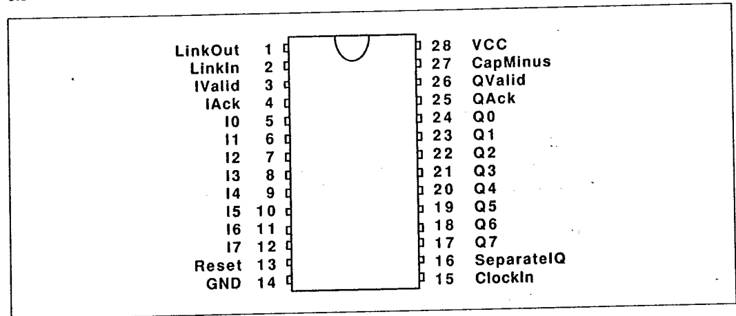
Figure 8.3: IMS C011 Mode 1 pinout
