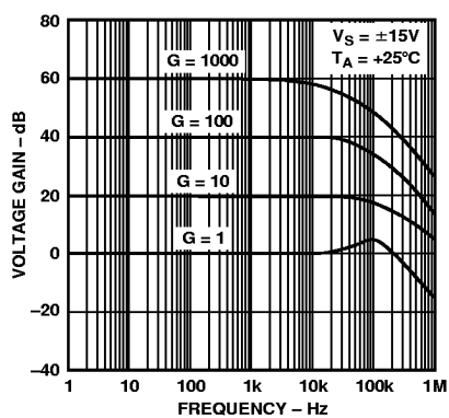
Figure 17. Closed-Loop Voltage Gain vs. Frequency
