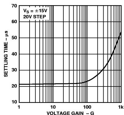
Figure 22. Settling Time to 0.01% vs. Voltage Gain
