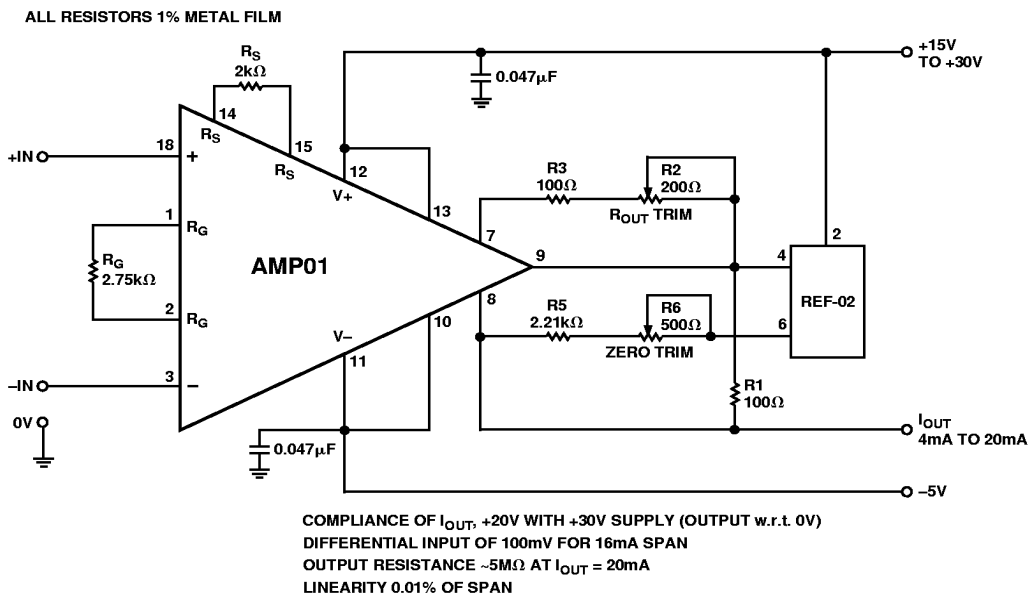
Figure 37. 13-Bit Linear 4-20 mA Transmitter Constructed by Adding a Voltage Reference. Thermocouple Signals Can Be Accepted Without Preamplification.
