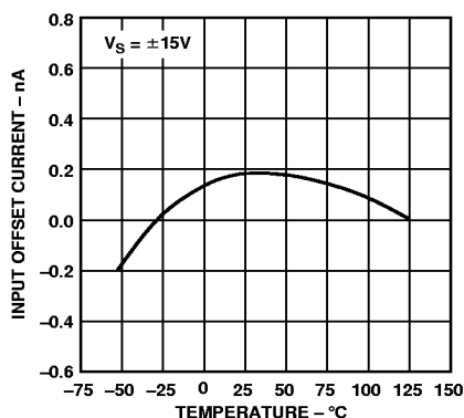
Figure 8. Input Offset Current vs. Temperature
