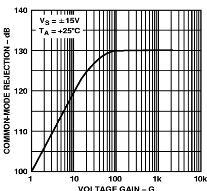
Figure 9. Common-Mode Rejection vs. Voltage Gain
