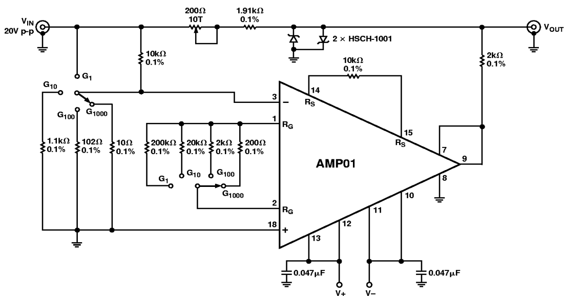
Figure 45. Settling-Time Test Circuit
