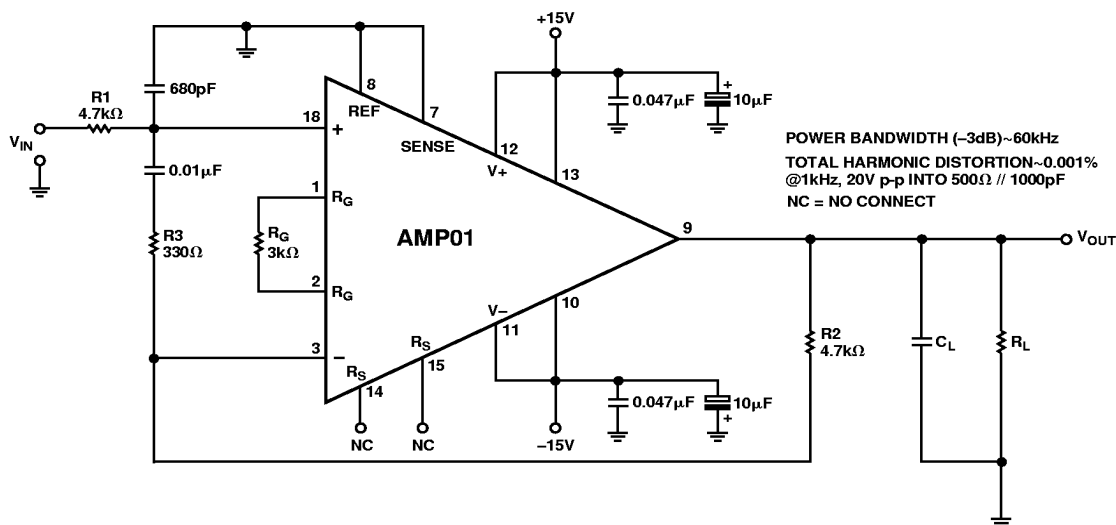
Figure 43. Stability with Large Capacitive Loads Combined with High Output Current Capability make the AMP01 Ideal for Line Driving Applications. Offset Voltage Drift Approaches the TCV_{IOS} Limit, (0.3 μV/°C).
