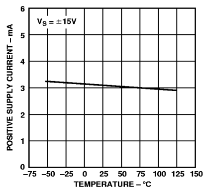
Figure 27. Positive Supply Current vs. Temperature
