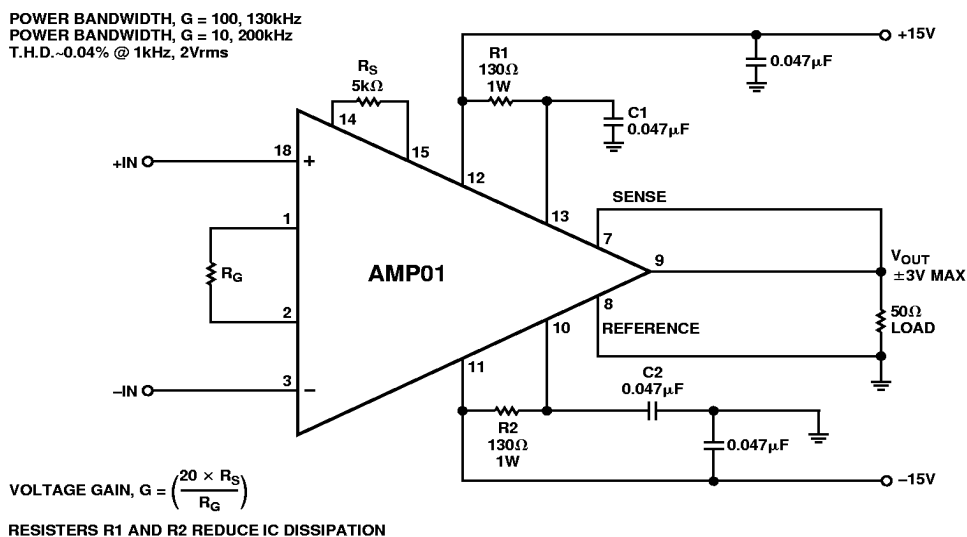
Figure 34. Driving 50 \Omega Loads
