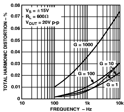
Figure 18. Total Harmonic Distortion vs. Frequency
