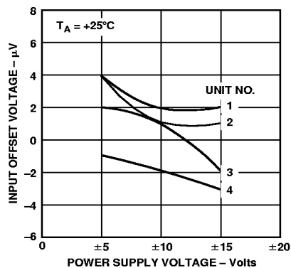
Figure 3. Input Offset Voltage vs. Supply Voltage
