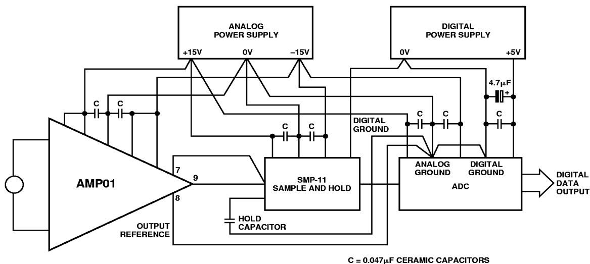
Figure 32. Basic Grounding Practice
