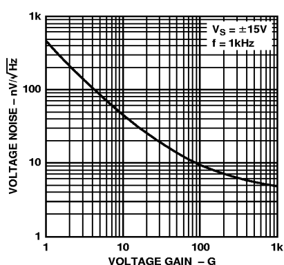
Figure 24. RTI Voltage Noise Density vs. Gain
