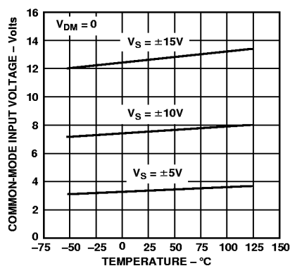
Figure 11. Common-Mode Voltage Range vs. Temperature
