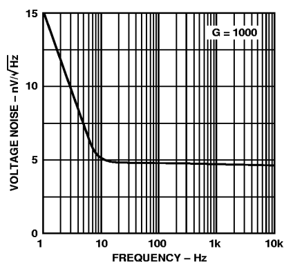
Figure 23. Voltage Noise Density vs. Frequency
