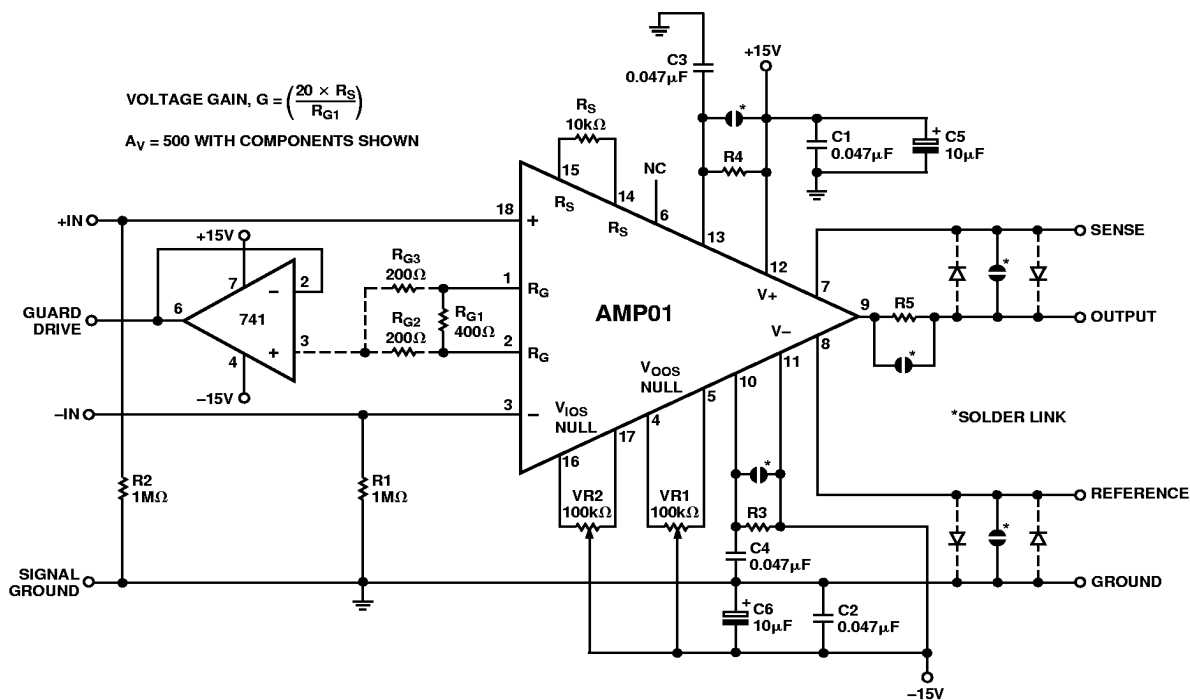
Figure 31. AMP01 Evaluation Circuit Showing Guard-Drive Connection
