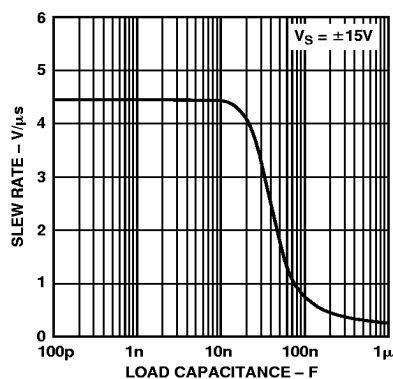
Figure 21. Slew Rate vs. Load Capacitance
