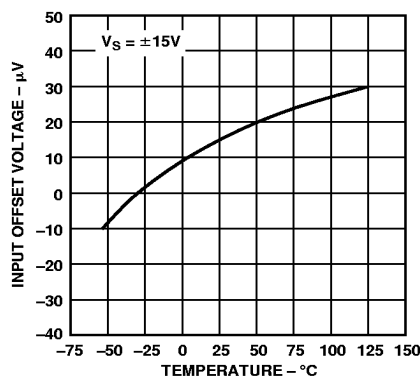
Figure 2. Input Offset Voltage vs. Temperature
