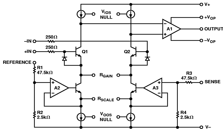
Figure 1. Simplified Schematic
