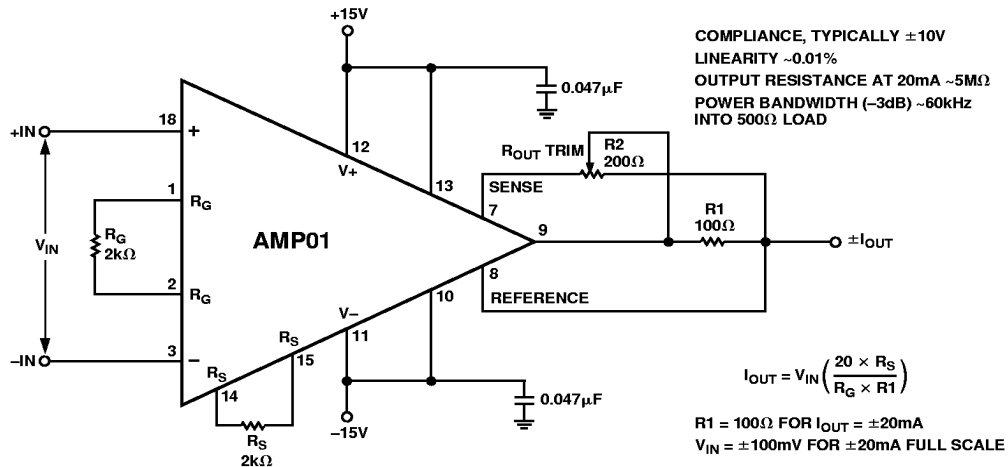
Figure 36. High Compliance Bipolar Current Source with 13-Bit Linearity
