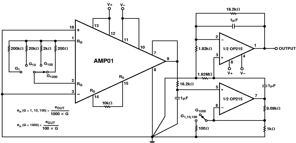
Figure 44. Noise Test Circuit (0.1 Hz to 10 Hz)
