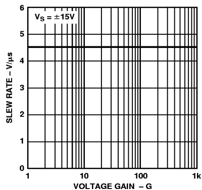
Figure 20. Slew Rate vs. Voltage Gain
