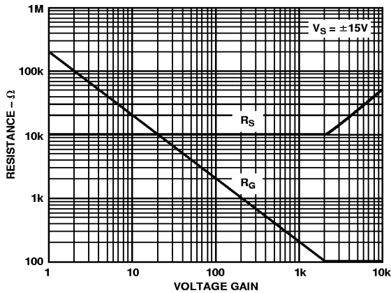
Figure 30. R_G and R_S Selection
