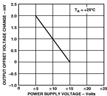
Figure 5. Output Offset Voltage Change vs. Supply Voltage
