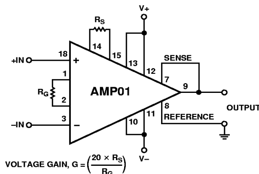
Figure 29. Basic AMP01 Connections for Gains 0.1 to 10,000
