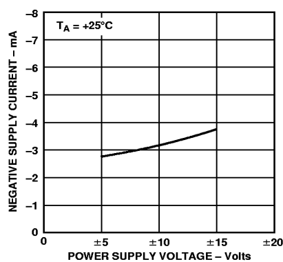
Figure 26. Negative Supply Current vs. Supply Voltage
