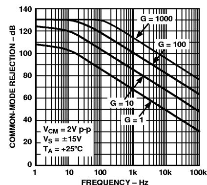
Figure 10. Common-Mode Rejection vs. Frequency
