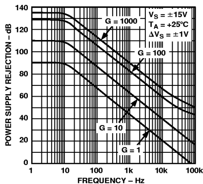
Figure 12. Positive PSR vs. Frequency
