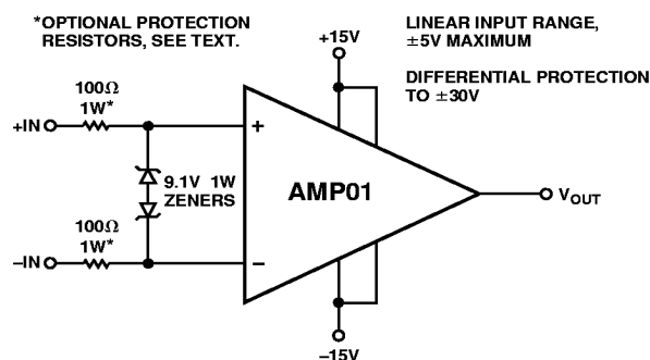
Figure 35. Input Overvoltage Protection for Gains 2 to 10,000
