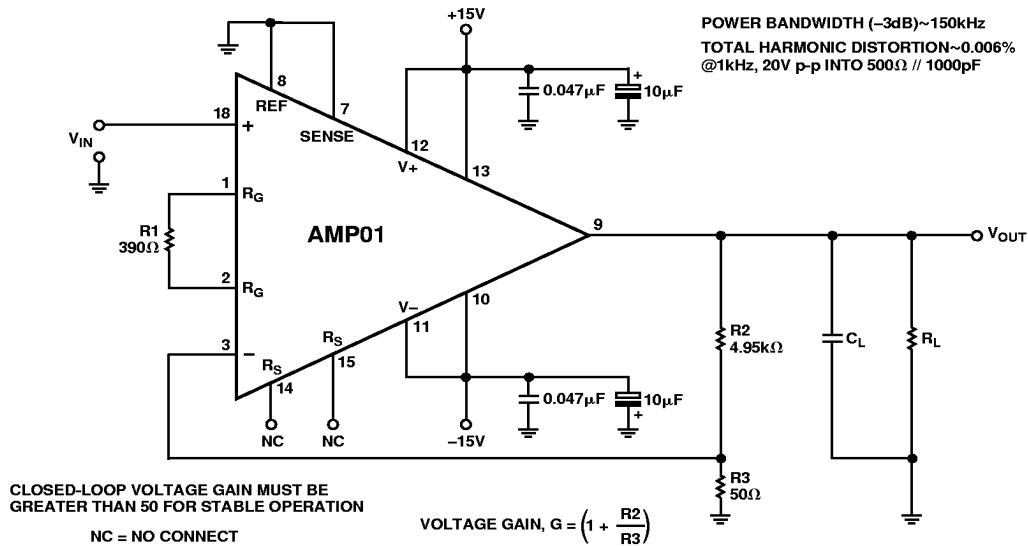
Figure 41. Configuring the AMP01 as a Noninverting Operational Amplifier Provides Exceptional Performance. The Output Handles Low Load Impedances at Very Low Distortion, 0.006%.
