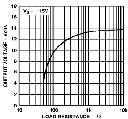
Figure 14. Maximum Output Voltage vs. Load Resistance
