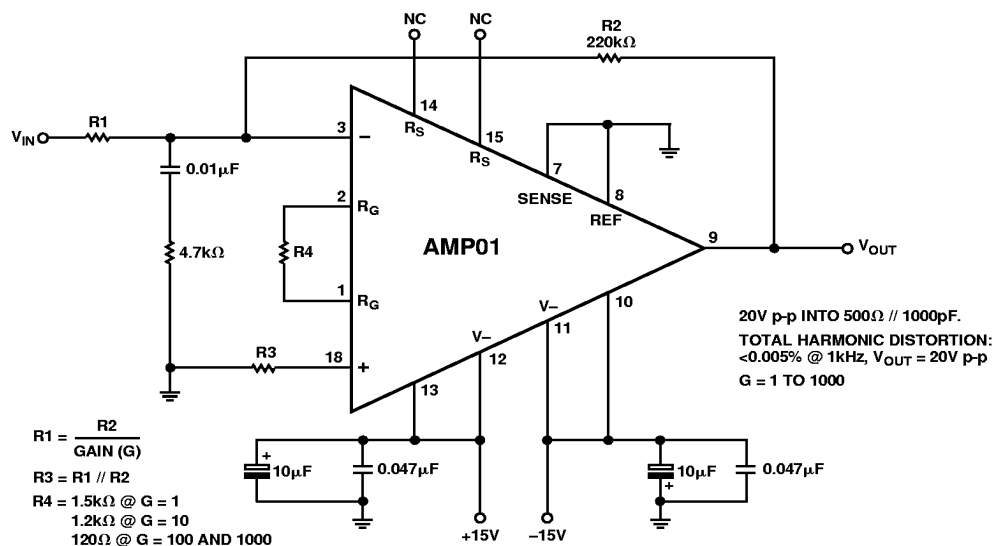
Figure 42. The Inverting Operational Amplifier Configuration has Excellent Linearity over the Gain Range 1 to 1000, Typically 0.005%. Offset Voltage Drift at Unity Gain Is Improved over the Drift in the Instrumentation Amplifier Configuration.
