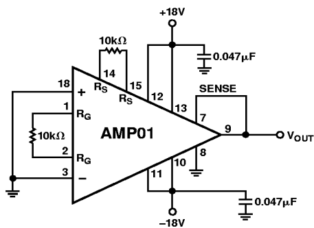
Figure 47. Burn-In Circuit
