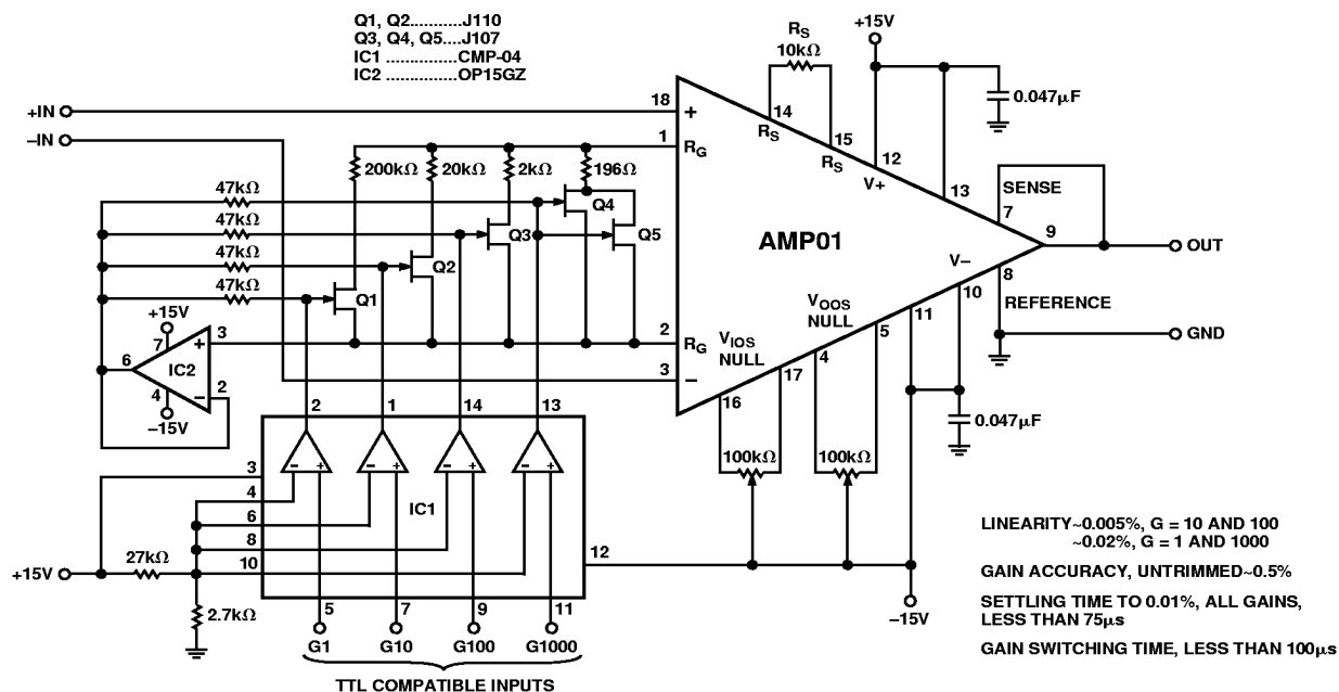
Figure 39. The AMP01 Makes an Excellent Programmable-Gain Instrumentation Amplifier. Combined Gain-Switching and Settling Time to 13 Bits Falls Below 100 μs. Linearity Is Better than 12 Bits over a Gain Range 1 to 1000.
