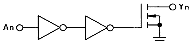
FIGURE 3. Logic diagram.
