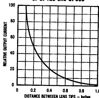
Coupling Characteristics of OP123 and OP300
