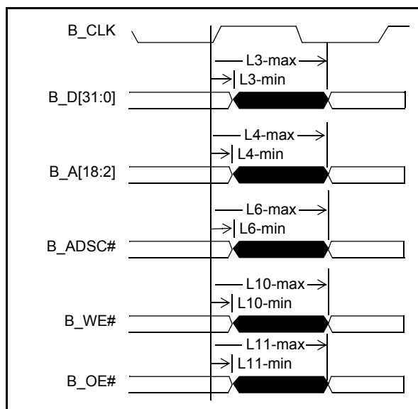
Figure 11 - Local Memory Interface - Output valid delay timing
