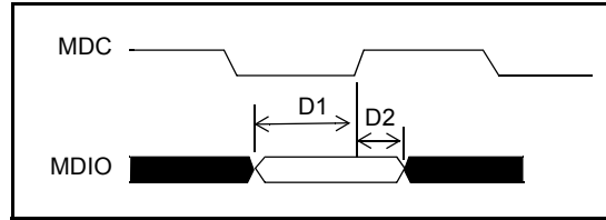
Figure 19 - MDIO Input Setup and Hold Timing
