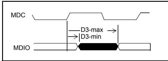
Figure 20 - MDIO Output Delay Timing
