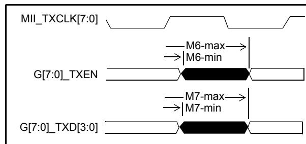
Figure 12 - AC Characteristics – Media Independent Interface
