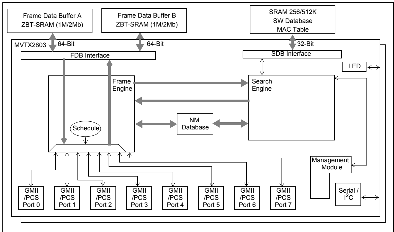
Figure 1 - MVTX2803AG Block Diagram
