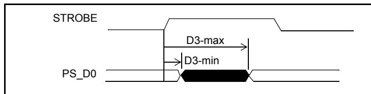
Figure 24 - Serial Interface Output Delay Timing
