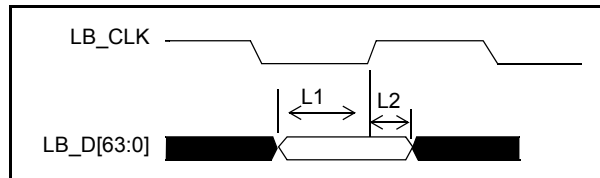
Figure 8 - Local Memory Interface – Input setup and hold timing
