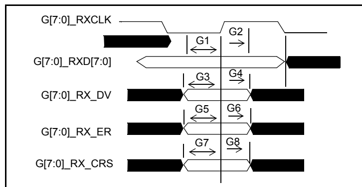
Figure 15 - AC Characteristics – Gigabit Media Independent Interface
