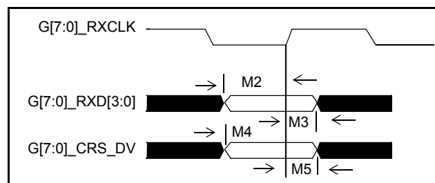
Figure 13 - AC Characteristics – Media Independent Interface
