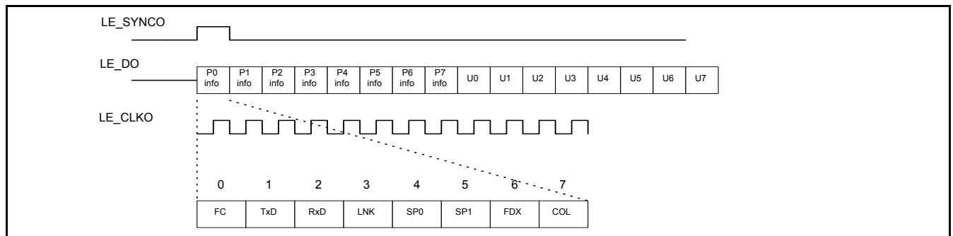
Figure 5 - Timing diagram for serial mode in LED interface
