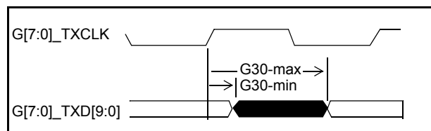
Figure 16 - AC Characteristics – PCS Interface
