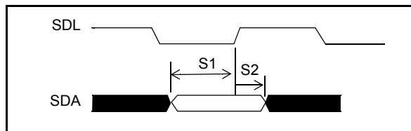
Figure 21 - I 2 C Input Setup Timing
