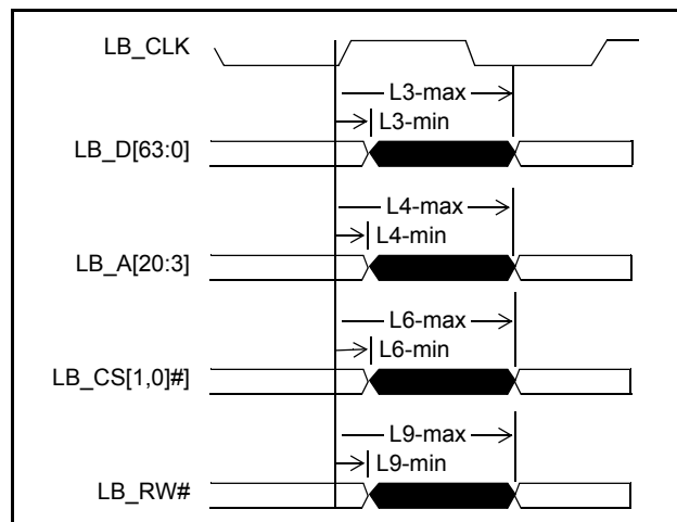
Figure 9 - Local Memory Interface - Output valid delay timing
