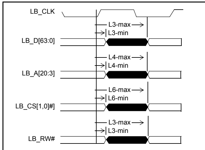
Figure 7 - Local Memory Interface - Output valid delay timing
