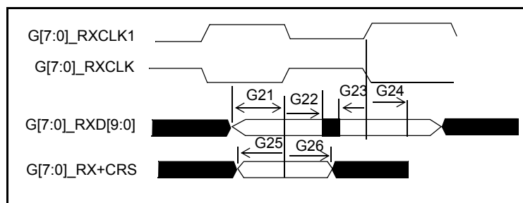
Figure 17 - AC Characteristics – PCS Interface
