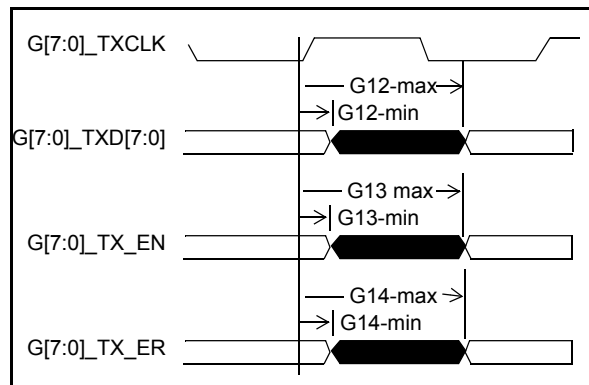
Figure 14 - AC Characteristics- GMII
