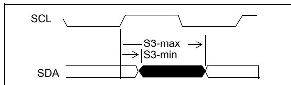
Figure 22 - I 2 C Output Delay Timing
