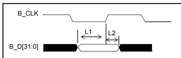
Figure 10 - Local Memory Interface – Input setup and hold timing
