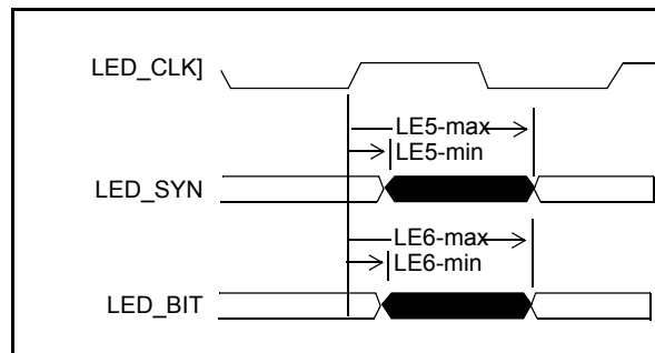
Figure 18 - AC Characteristics – LED Interface
