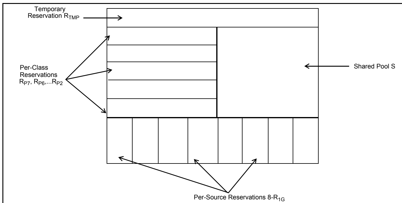
Figure 4 - Buffer Partition Scheme Used in the MVTX2803AG
