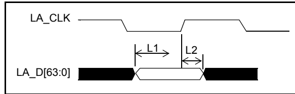
Figure 6 - Local Memory Interface – Input setup and hold timing
