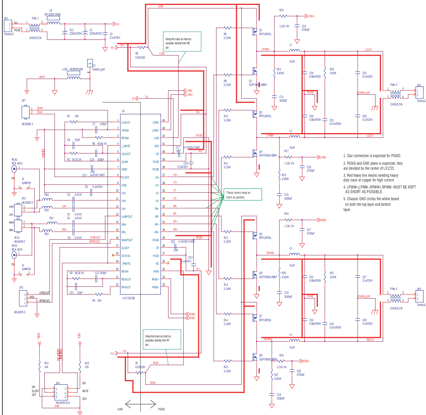
FIGURE 1 - LXE1722-150 SCHEMATIC
