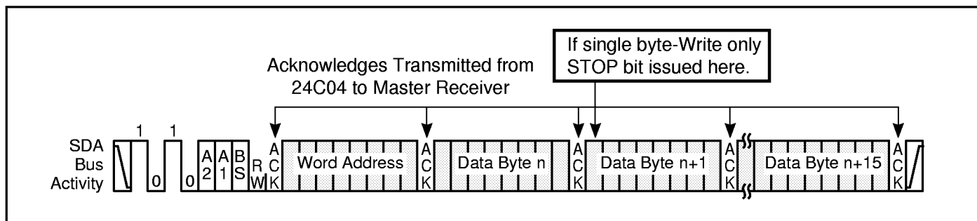
Figure 6. Write Operation
