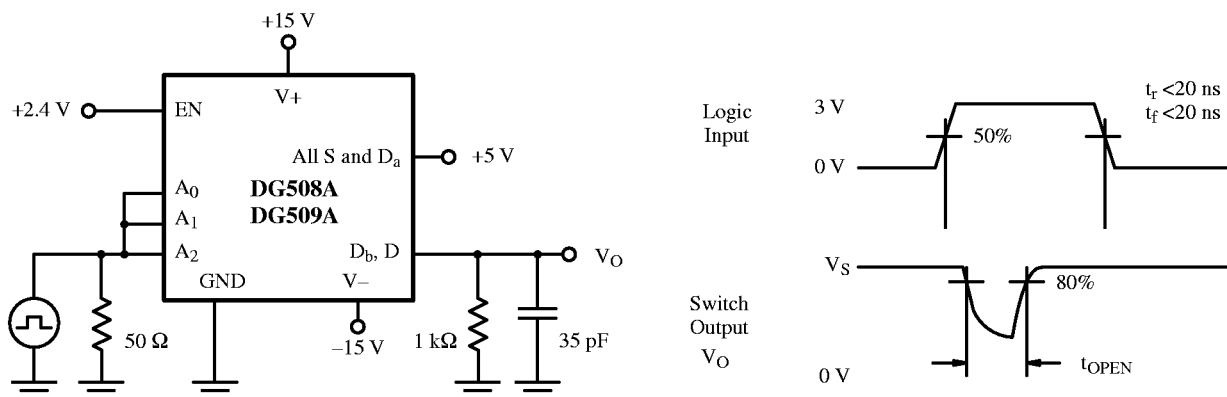
Figure 4. Break-Before-Make Interval
