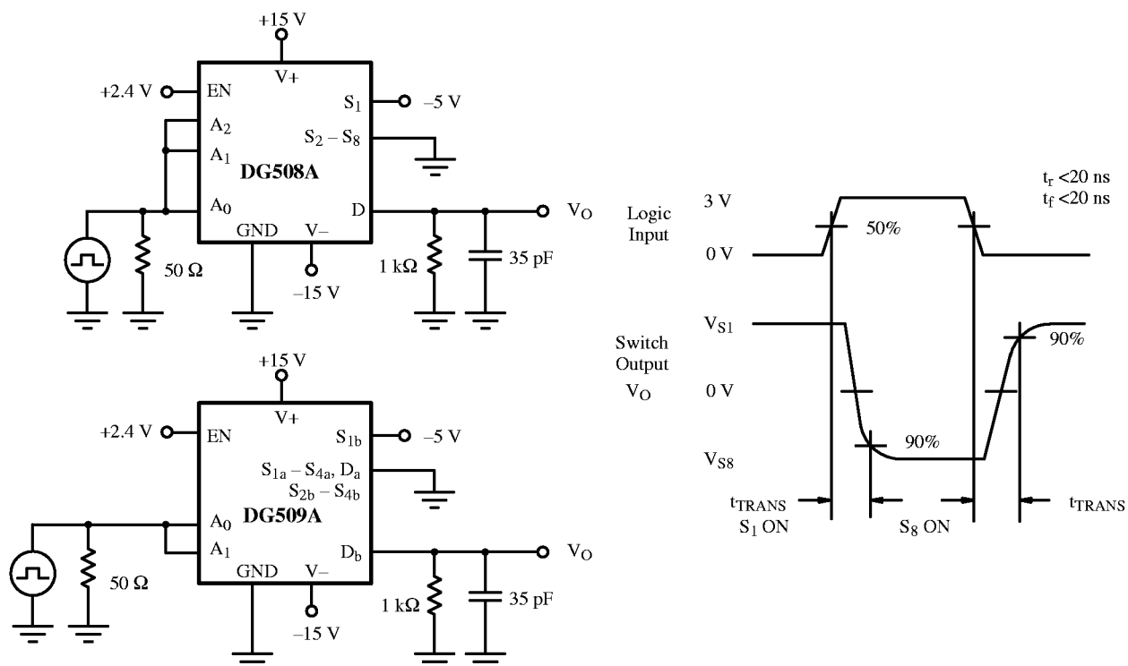
Figure 2. Transition Time
