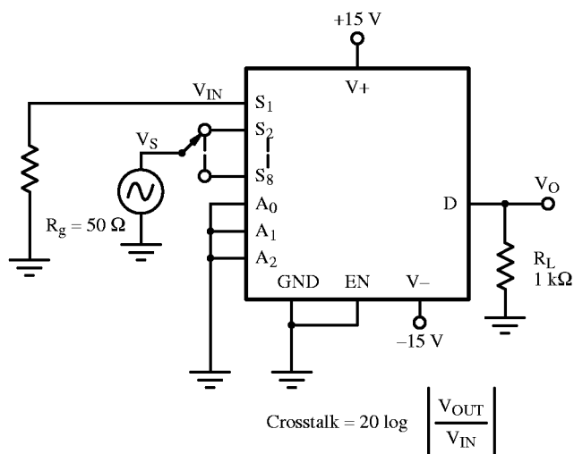
Figure 7. Crosstalk
