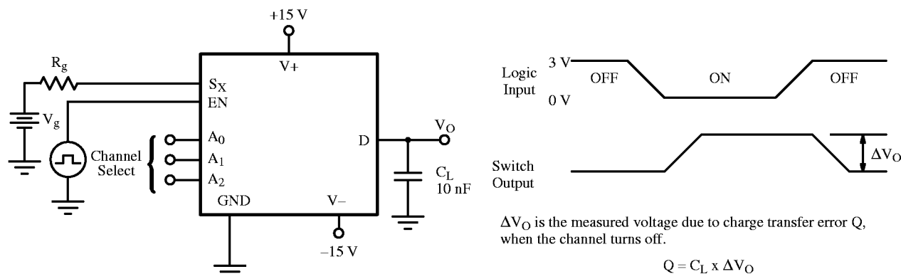
Figure 5. Charge Injection
