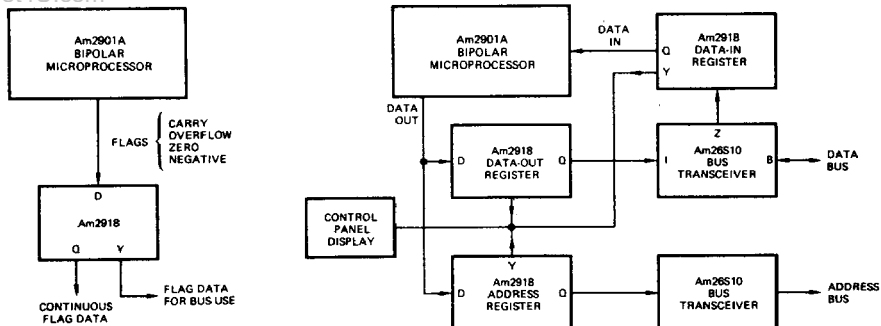
The Am2918 used as data-in, data-out and address registers.
