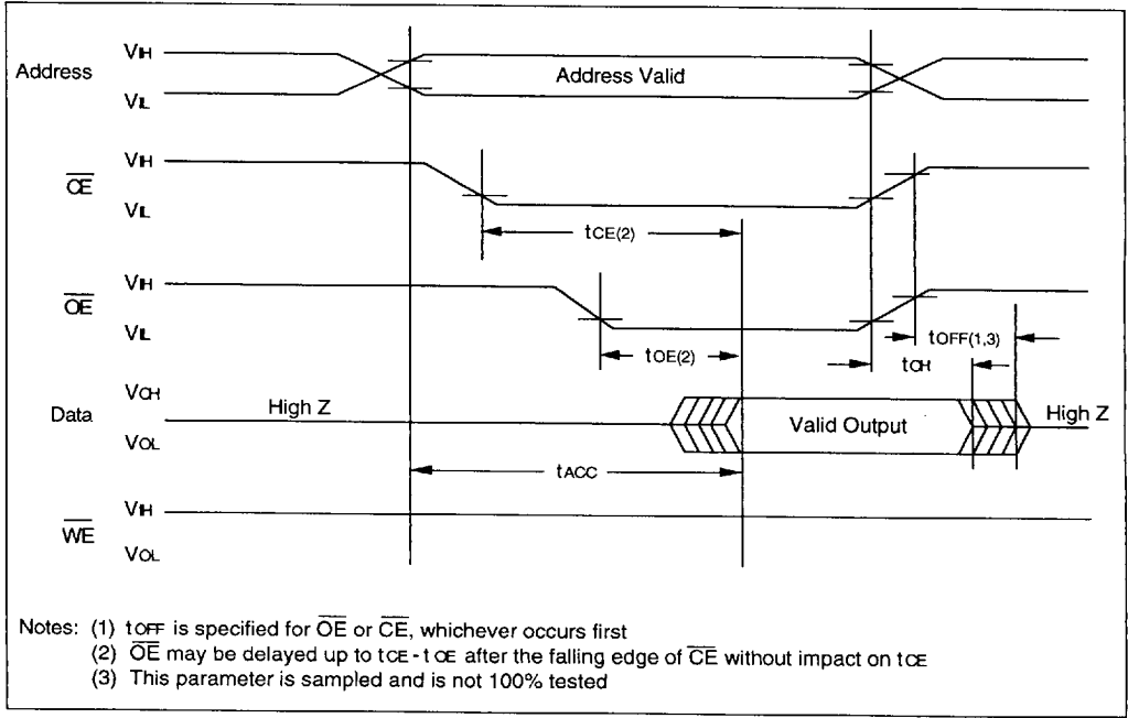
FIGURE 1-1: READ WAVEFORMS
