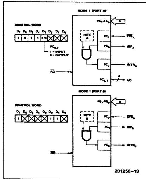
Figure 8. MODE 1 input
