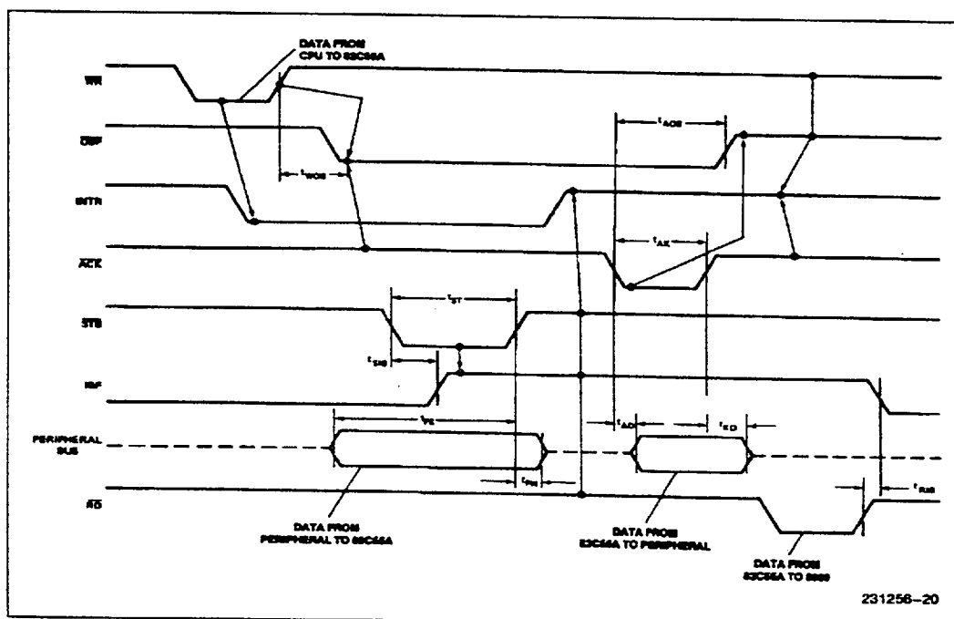
Figure 15. MODE 2 (Bidirectional)
