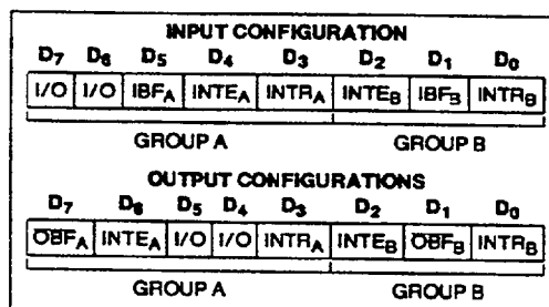
Figure 17a. MODE 1 Status Word Format
