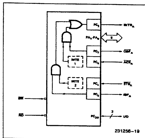
Figure 14. MODE 2
