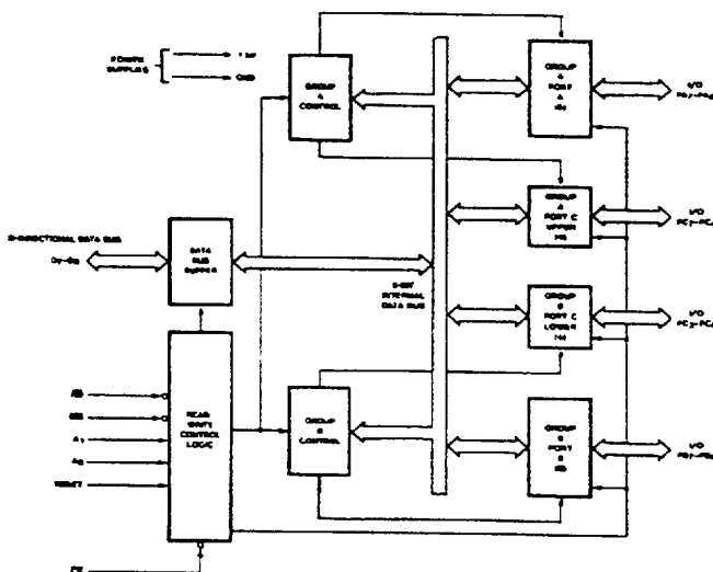
Figure 1. 82C55A Block Diagram
