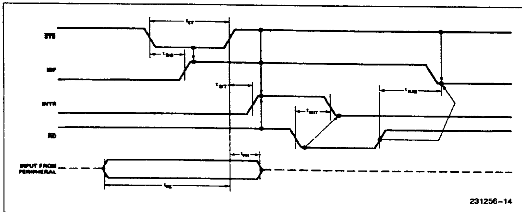
Figure 9. MODE 1 (Strobed Input)
