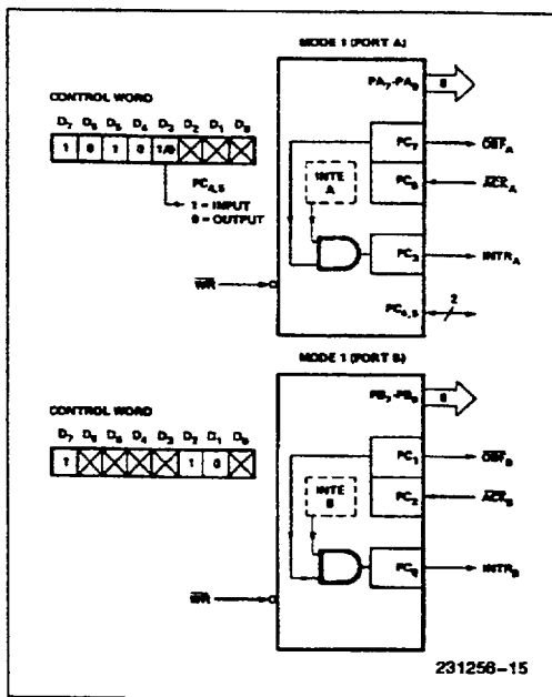
Figure 10. MODE 1 Output
