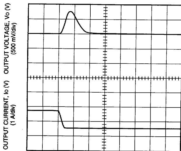
Figure 14. Typical JW150H Transient Response to Step Decrease in Load from 50% to 25% of Full Load at Room Temperature and 48 V Input (Waveform Averaged to Eliminate Ripple Component.)
