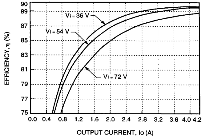
Figure 11. Typical JW100H Converter Efficiency vs. Output Current at Room Temperature
