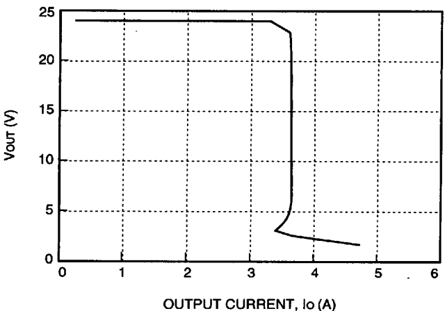
Figure 6. Typical JW075H Output Characteristics at Room Temperature, V_{IN} = 48 V
