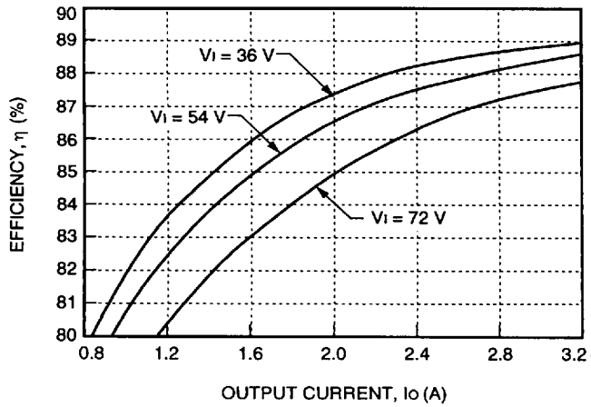
Figure 10. Typical JW075H Converter Efficiency vs. Output Current at Room Temperature
