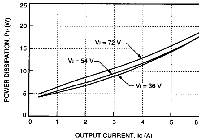
Figure 31. JW150H Power Dissipation vs. Output Current
