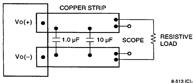
Figure 17. Input Reflected-Ripple Test Setup
