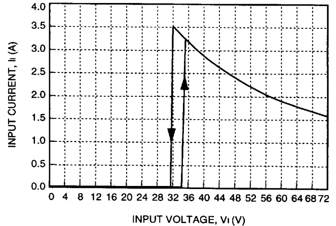
Figure 3. Typical JW100H Input Characteristics at Room Temperature, I_o = 4.2 A
