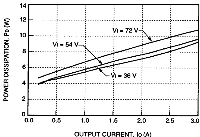
Figure 29. JW075H Power Dissipation vs. Output Current
