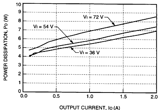
Figure 28. JW050H Power Dissipation vs. Output Current
