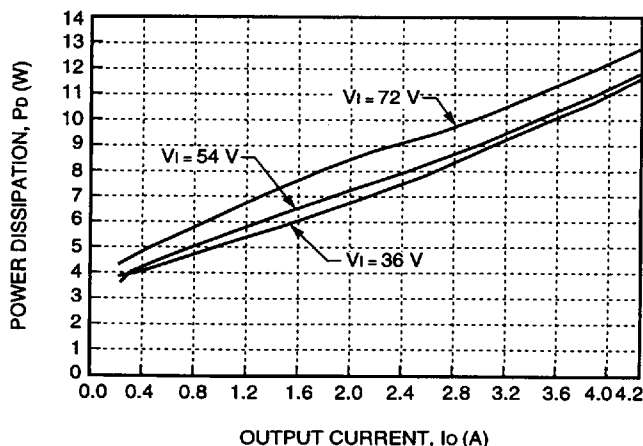
Figure 30. JW100H Power Dissipation vs. Output Current
