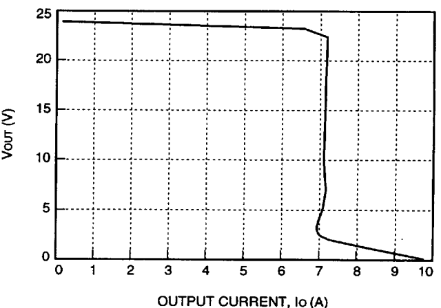
Figure 8. Typical JW150H Output Characteristics at Room Temperature, V_{IN} = 48 V
