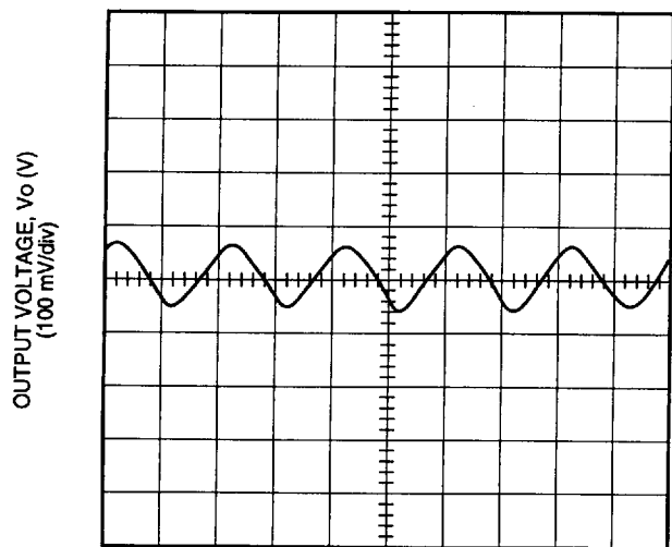
Figure 13. Typical JW150H Output Ripple Voltage at Room Temperature, 48 V Input, I_o = Full Load
