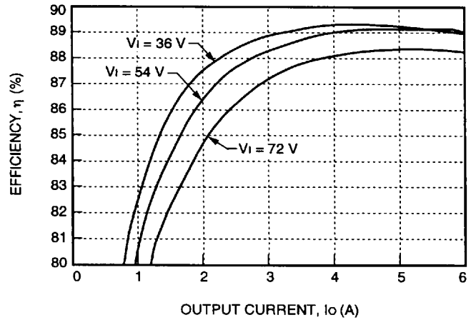
Figure 12. Typical JW150H Converter Efficiency vs. Output Current at Room Temperature
