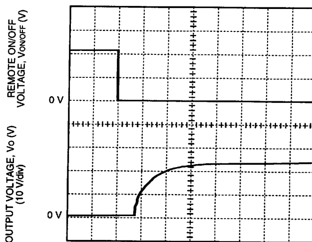
Figure 16. Typical Start-Up from Remote On/Off JW150H1; I_o = Full Load
