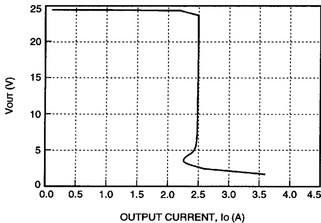
Figure 5. Typical JW050H Output Characteristics at Room Temperature, V_{IN} = 48 V
