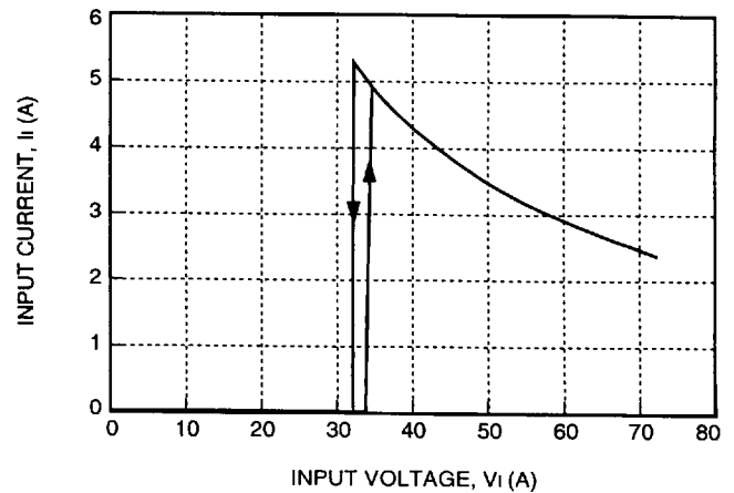
Figure 4. Typical JW150H Input Characteristics at Room Temperature, I_o = 6.2 A
