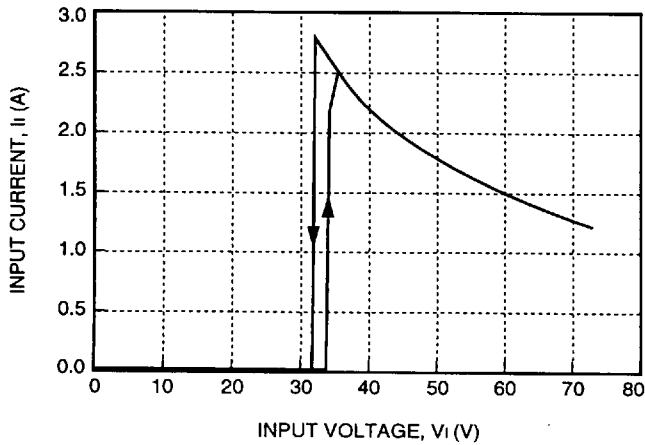
Figure 2. Typical JW075H Input Characteristics at Room Temperature, I_o = 3.1 A
