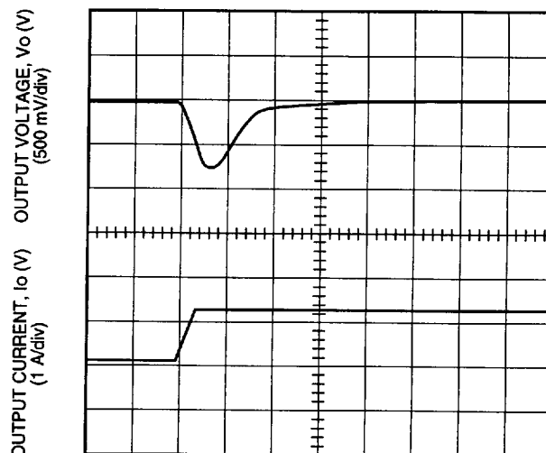
Figure 15. Typical JW150H Transient Response to Step Increase in Load from 50% to 75% of Full Load at Room Temperature and 48 V Input (Waveform Averaged to Eliminate Ripple Component.)
