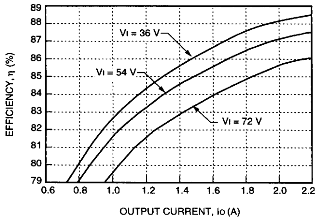
Figure 9. Typical JW050H Converter Efficiency vs. Output Current at Room Temperature
