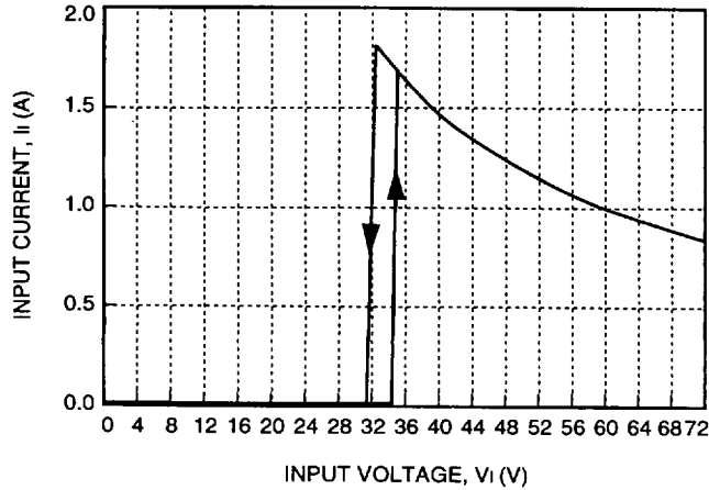
Figure 1. Typical JW050H Input Characteristics at Room Temperature, I_o = 2.1 A
