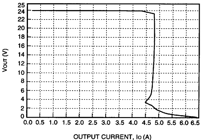
Figure 7. Typical JW100H Output Characteristics at Room Temperature, V_{IN} = 48 V
