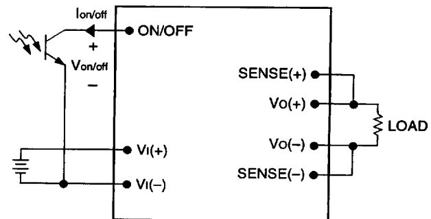
Figure 20. Remote On/Off Implementation 8-720 (C).c
