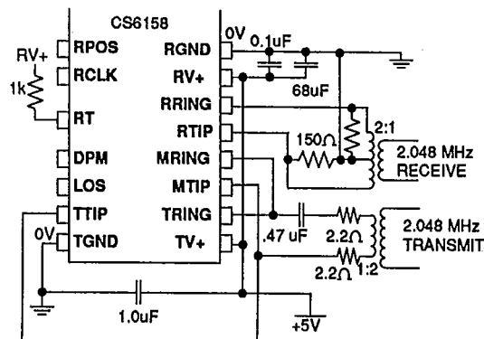
Figure A2. - Configuration for Transmitting onto 75 \Omega Coax
