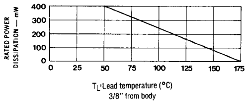
FIGURE 2 POWER DERATING CURVE
