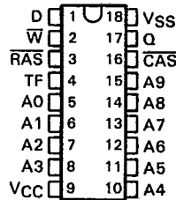
N PACKAGE (TOP VIEW)
