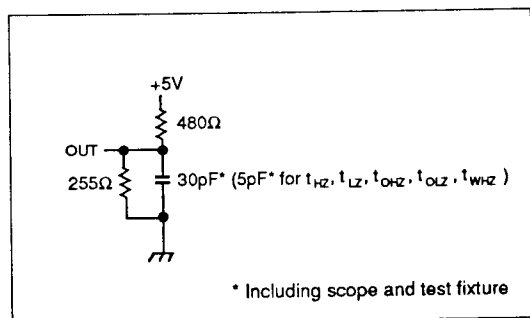
Figure 1. Output Load
