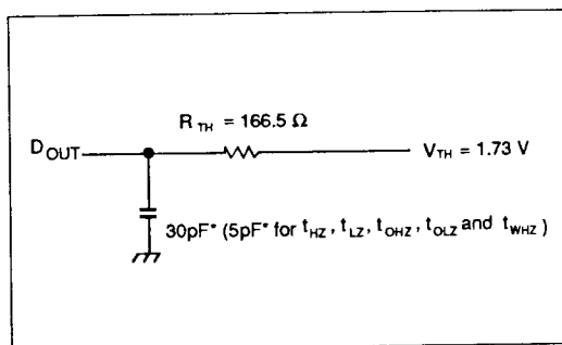
Figure 2. Thevenin Equivalent
