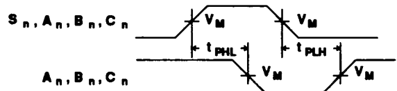
Waveform 2. Propagation Delay, Select And Data Busses
