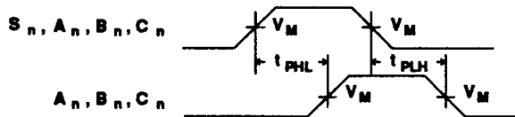
Waveform 1. Propagation Delay, Select And Data Busses
