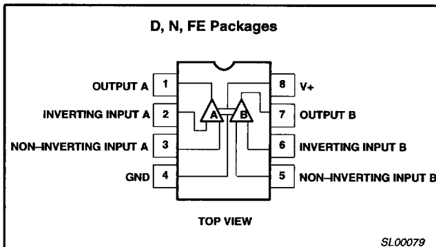
Figure 1. Pin Configuration
