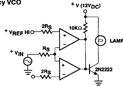
Limit Comparator
