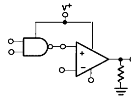
TTL-to-MOS Logic Converter
