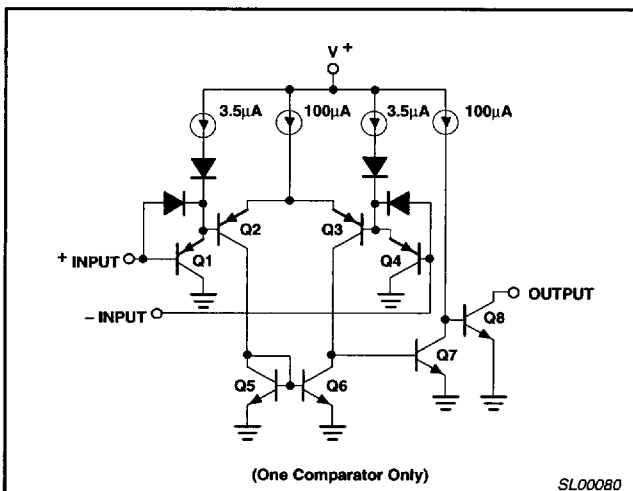
Figure 2. Equivalent Circuit
