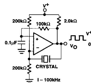
Crystal-Controlled Oscillator
