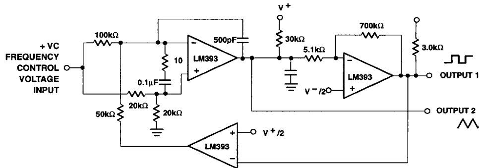
Two-Decade High-Frequency VCO
