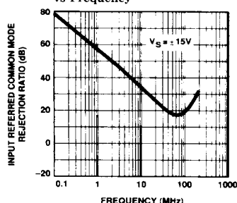
Input Referred Common Mode Rejection Ratio vs Frequency
