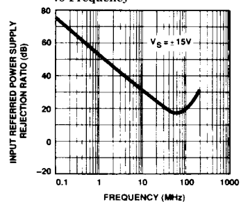
Input Referred Power Supply Rejection Ratio vs Frequency
