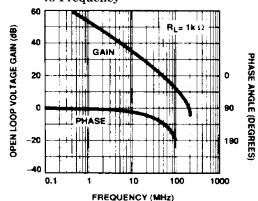
Open Loop Voltage Gain vs Frequency
