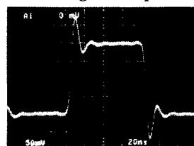
Small Signal Response
