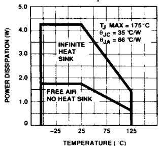
14-Lead CerDIP Maximum Power Dissipation vs Ambient Temperature
