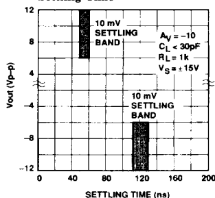
Settling Time
