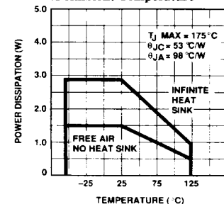
20-Lead LCC Maximum Power Dissipation vs Ambient Temperature
