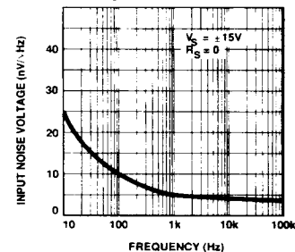
Input Noise Voltage vs Frequency
