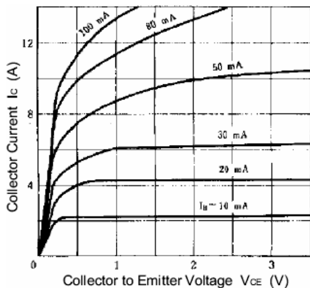
Fig.3 Static Characteristic
