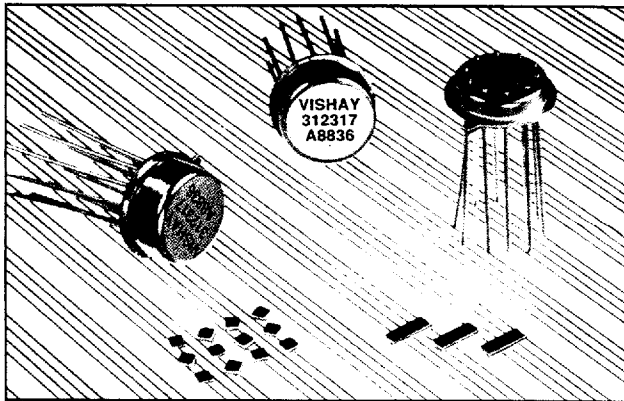
10 pins on a 0.230" pin circle—can contain up to 12 V5X5 resistor chips.
