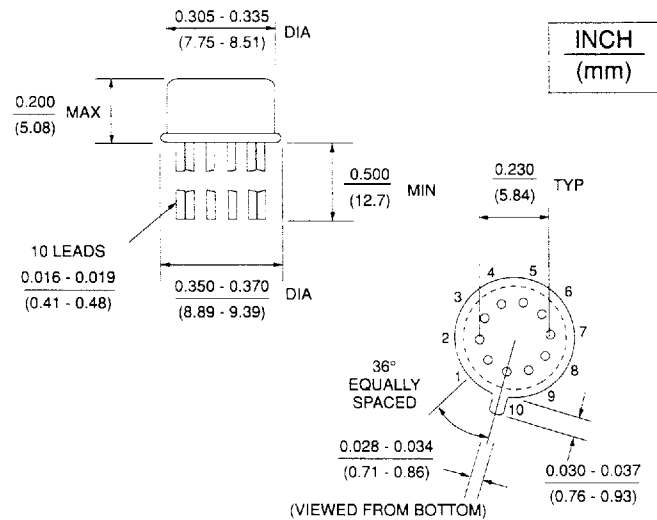
10 pins on a 0.230" pin circle—can contain up to 12 V5X5 resistor chips.
