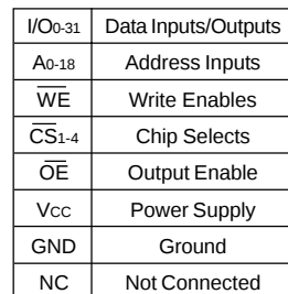
PIN DESCRIPTION
