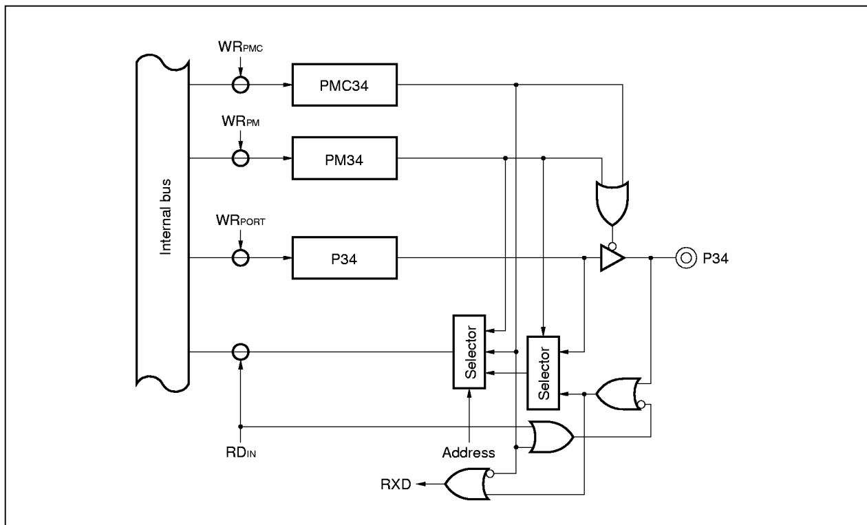
Figure 9-11. Block Diagram of P34 (Port 3)
