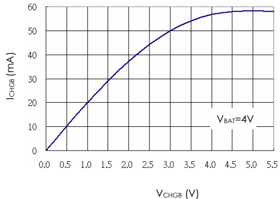
CHGB Pin I-V Curve (Strong Pull-Down State)
