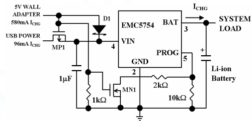
Figure 5. Combining Wall Adapter and USB Power
