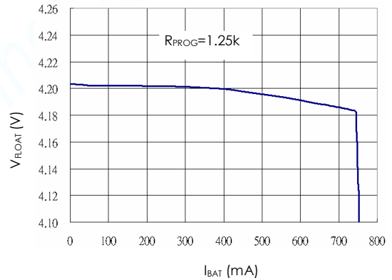
Regulated Output (Float) Voltage vs Charge Current
