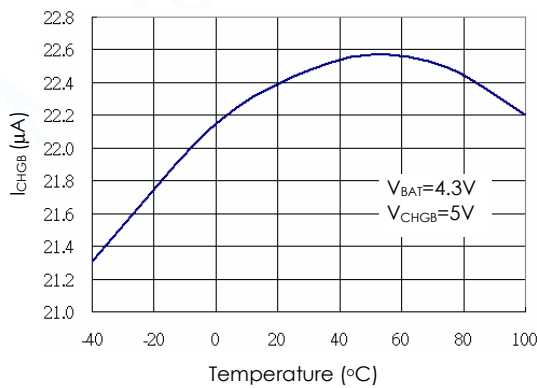
CHGB Pin Current vs Temperature (Weak Pull-Down State)
