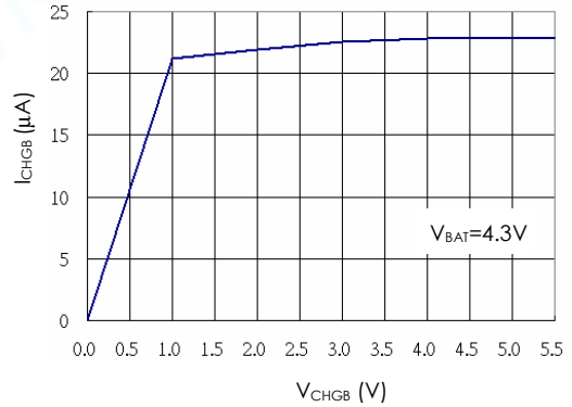
CHGB Pin I-V Curve (Weak Pull-Down State)
