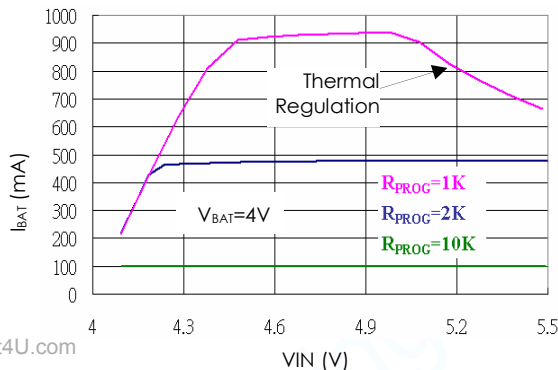
Charge Current vs Supply Voltage
