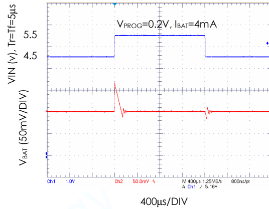
Line Transient (Battery Removed)
