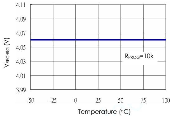
Recharge Voltage Threshold vs Temperature
