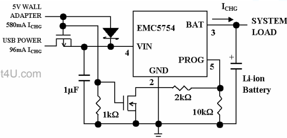
USB/Wall Adapter Power Li-ion Charger
