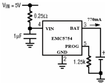
Li-ion Charger with External Power Dissipation
