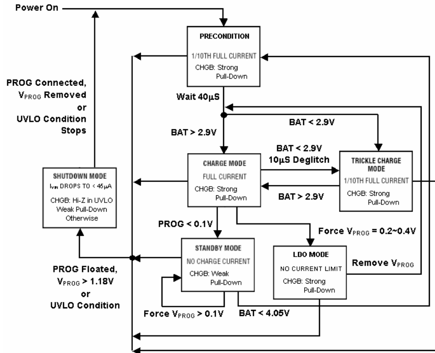
USB/Wall Adapter Power Li-ion Charger
