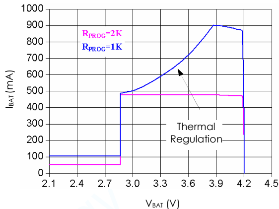
Charge Current vs Battery Voltage
