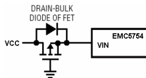
Figure 4. Low Loss Input Reverse Polarity Protection
