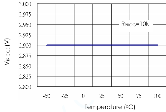
Trickle Charge Threshold vs Temperature
