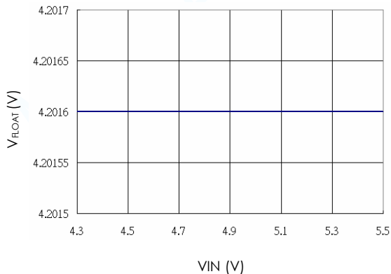
Regulated Output (Float) Voltage vs Supply Voltage
