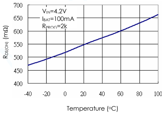
Power FET "ON" Resistance vs Temperature
