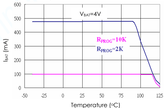
Charge Current vs Ambient Temperature
