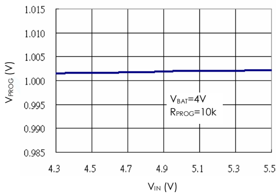
PROG Pin Voltage vs Supply Voltage (Constant Current Mode)
