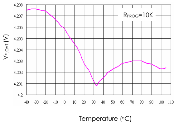
Regulated Output (Float) Voltage vs Temperature
