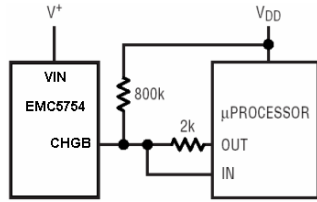
Figure 3. Using a Microprocessor to Determine CHGB State
