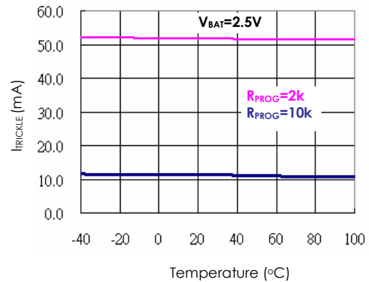
Trickle Charge Current vs Temperature
