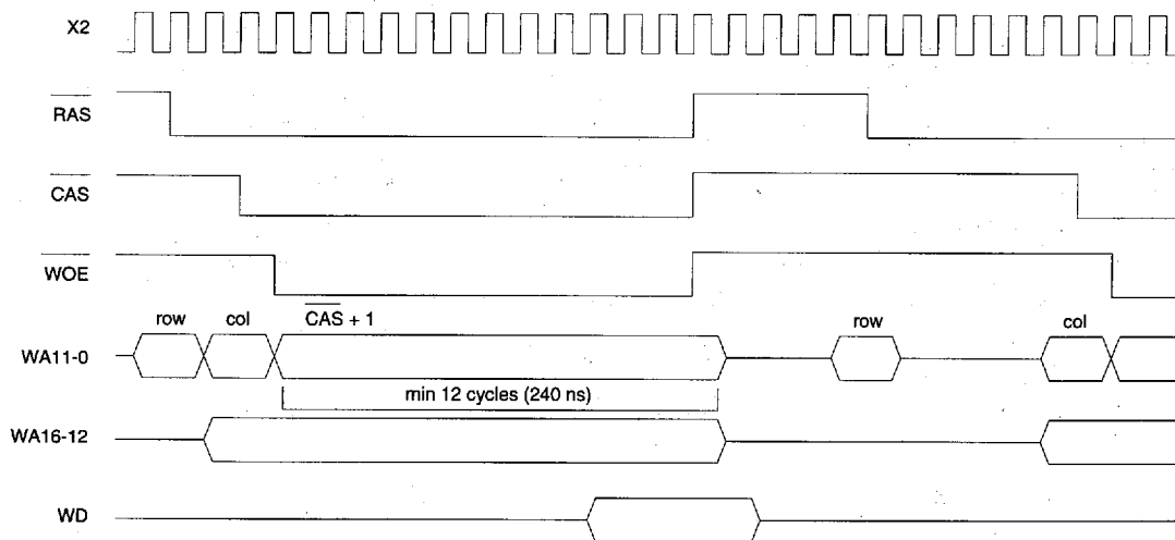
Figure 2. Typical External Memory Read Sequence
