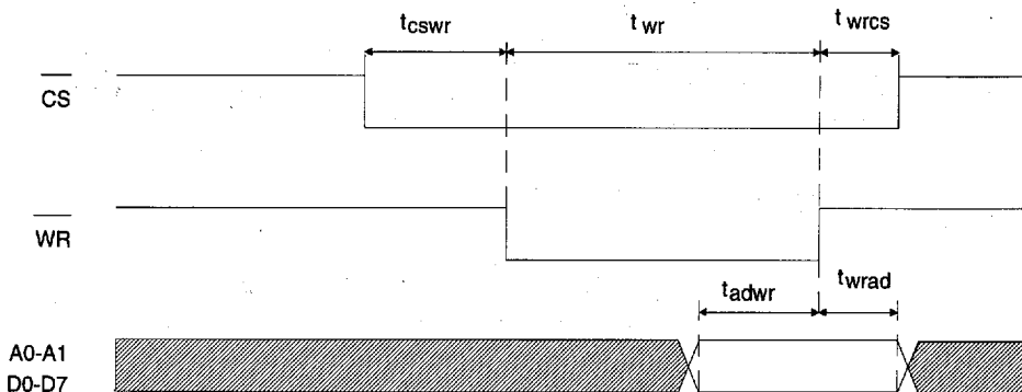
Microprocessor Write Cycle
