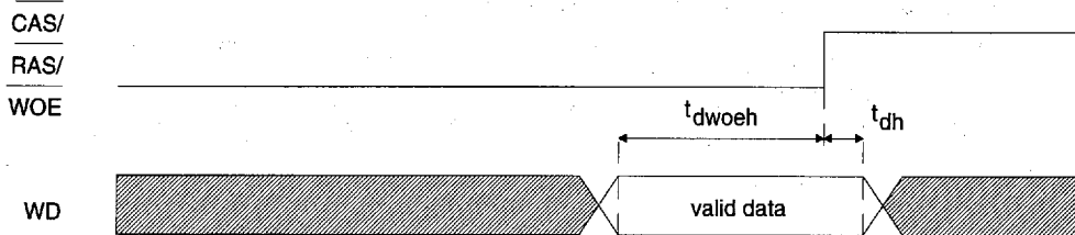
Sample Memory Data Bus Timing, Sample Memory Read
