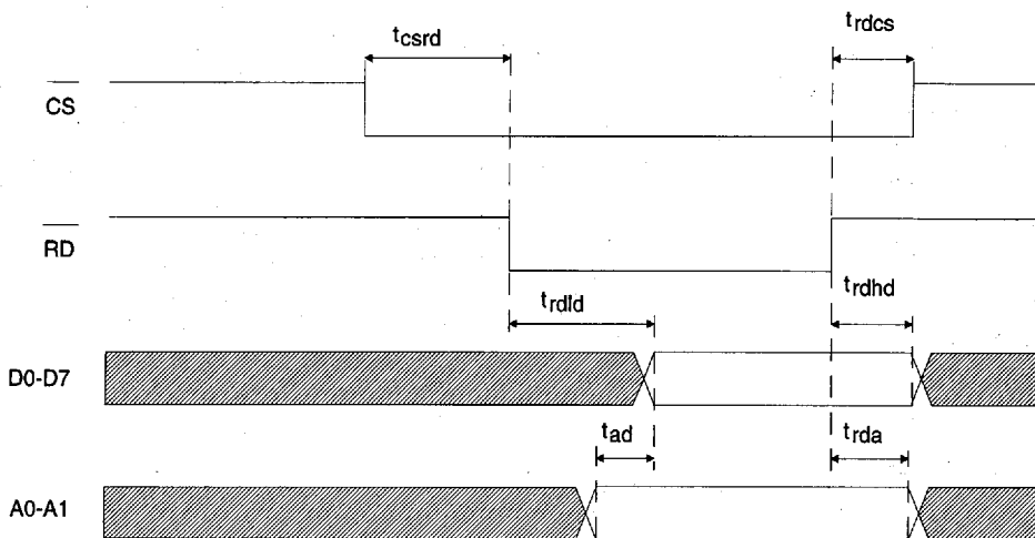
Microprocessor Read Cycle
