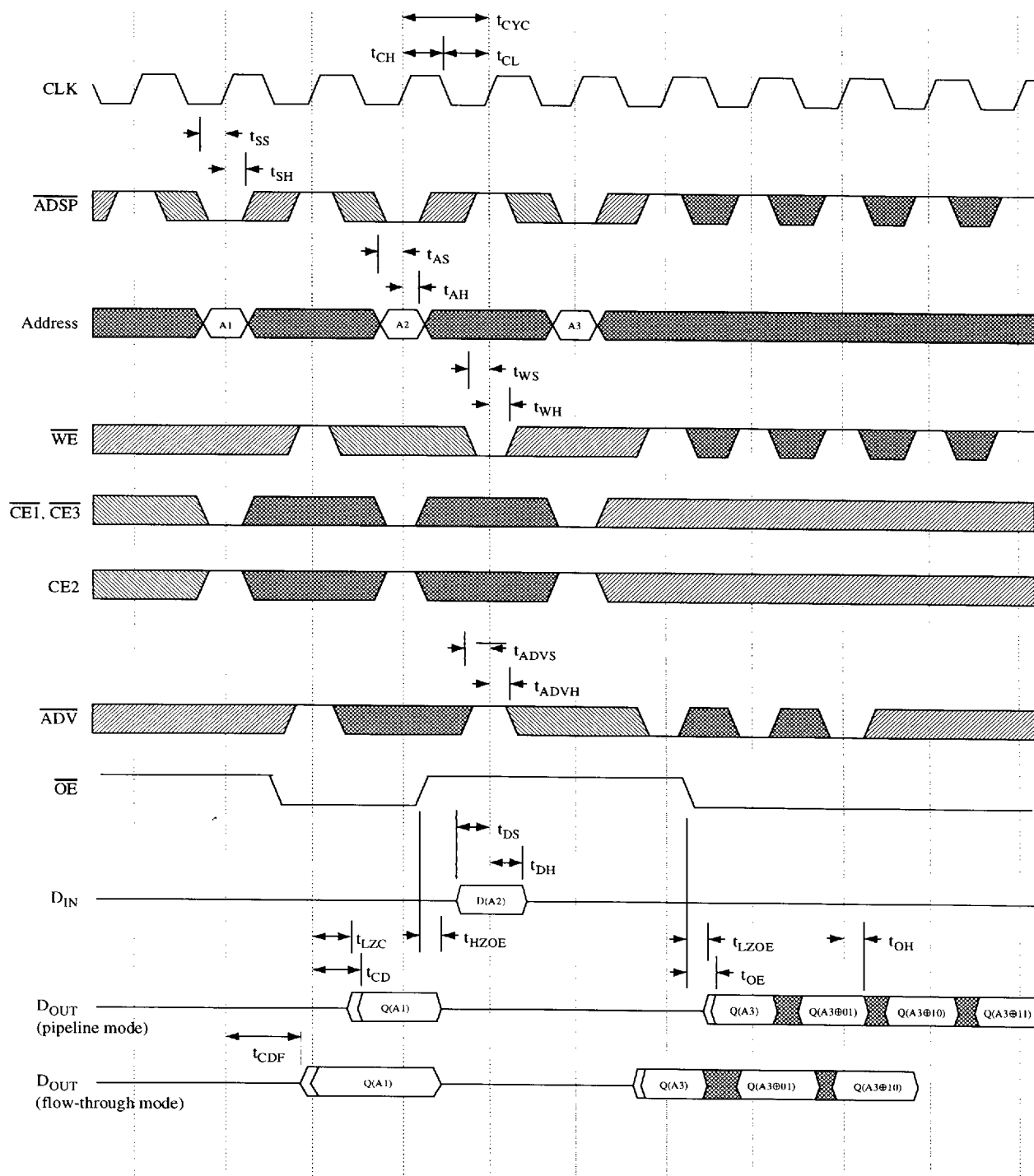
Timing waveform of read/write cycle
