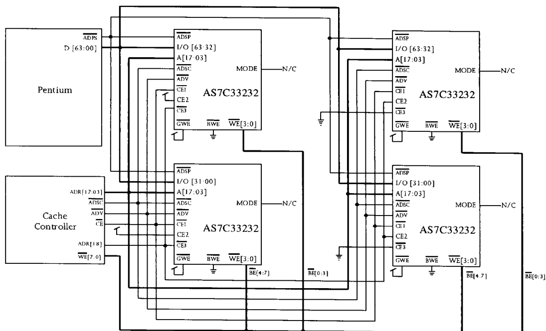
Figure B: Pentium 512KB two bank cache
