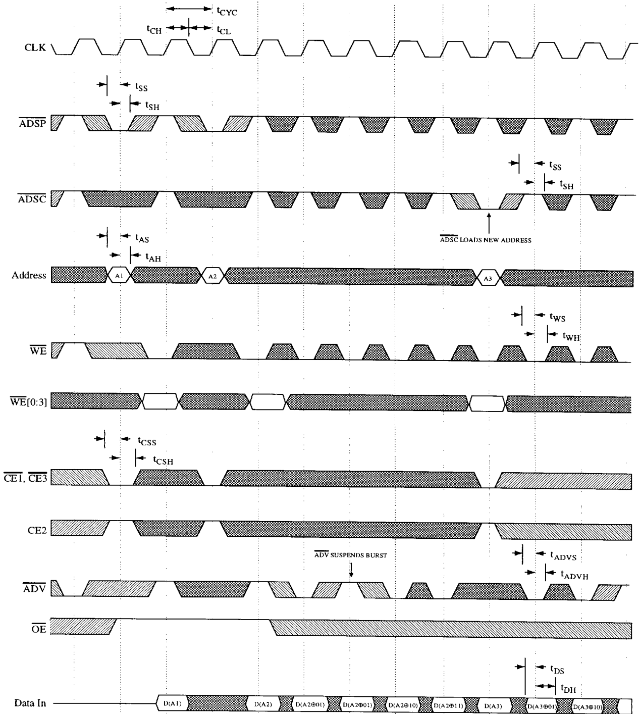
Timing waveform of write cycle
