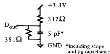
Figure C: Output Load (B) for t_{LZC} , t_{LZO\bar{E}} , t_{HZO\bar{E}} , t_{HZC}
