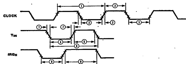
Figure 16. Additional Timing
