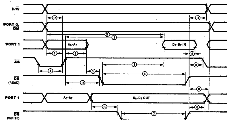
Figure 15. External I/O or Memory Read/Write
