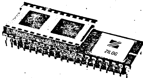
Figure 11. The Z8 Microcomputer Protopack Emulator
