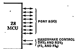
Figure 8c. Port 2
