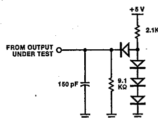
Figure 14. Test Load 1
