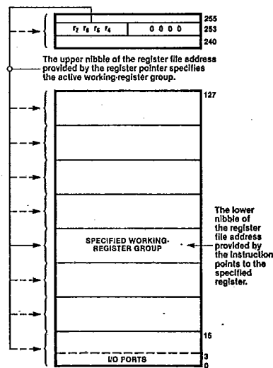
Figure 7. The Register Pointer
