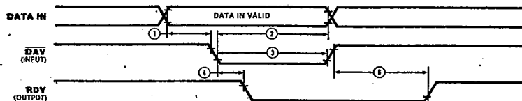
Figure 18a. Input Handshake
