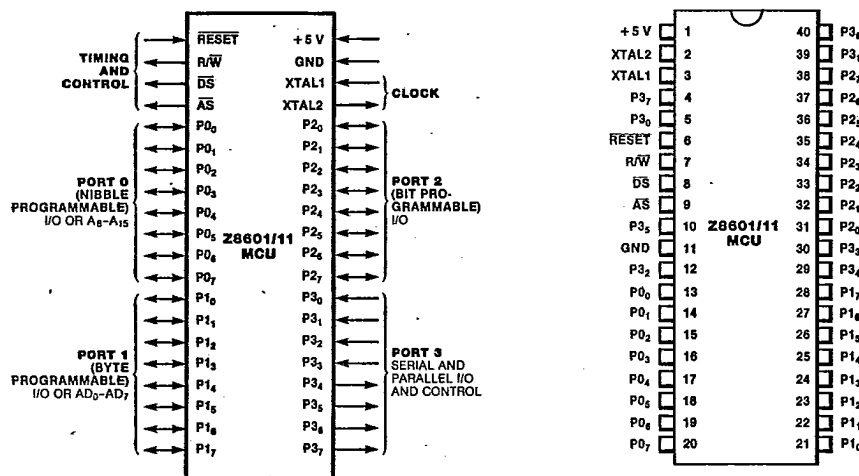
Figure 2a. 40-pin Dual-In-Line Package (DIP), Pin Assignments
