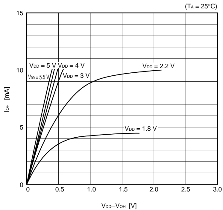
I_{OH} vs V_{DD}-V_{OH} (Ports 2, 3, 6, 8 and 9)
