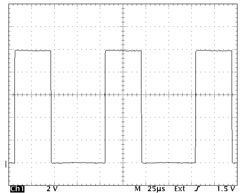
Typical Output Waveform, 10KHz, 10,000V, 120pF Load
