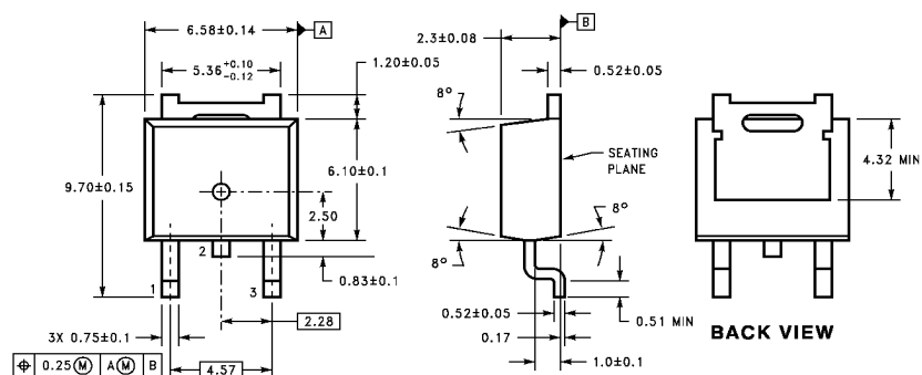
TO-252 Package (DT) NS Package Number TD03B
