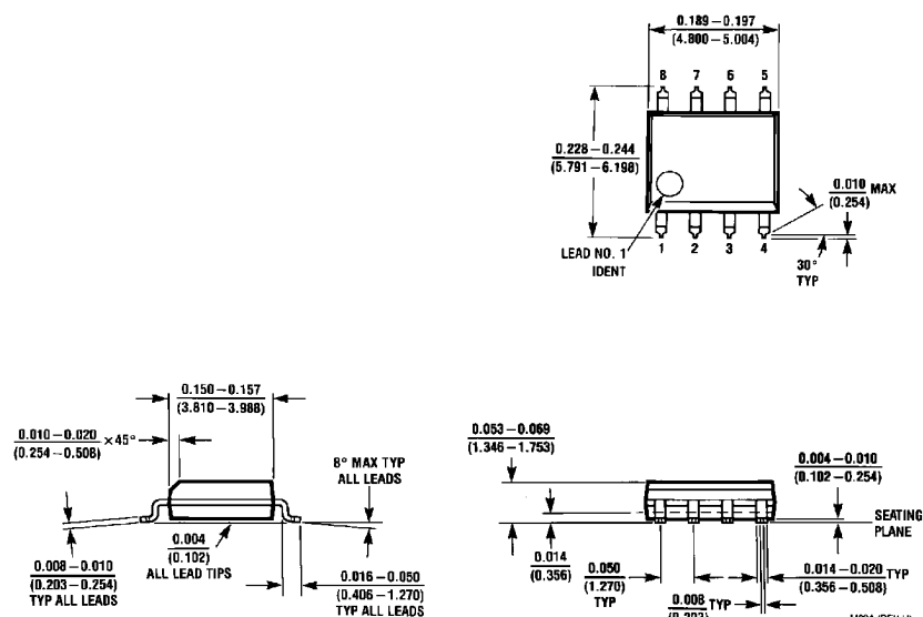
8-Lead Small Outline Molded Package (M) NS Package Number M08A
