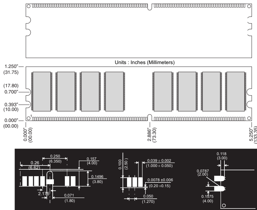
Figure 1: KVR400X64C3A/256 184-Pin DDR SDRAM Module
