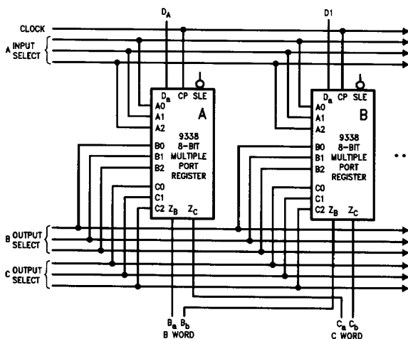
FIGURE a. Parallel Expansion
