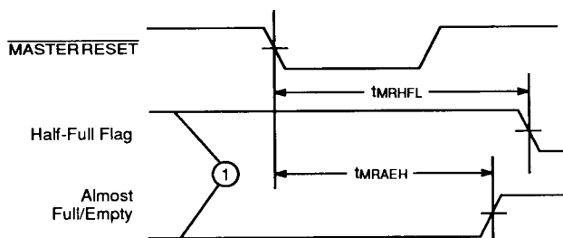
Figure 8. Master Reset Timing
