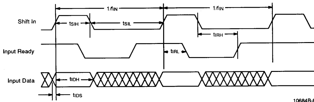
Figure 1. Input Timing
