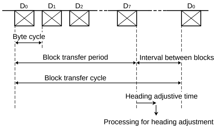
Fig. 2.3.25 Timing chart [Cyclic transmission or reception of block data between microcomputers]
